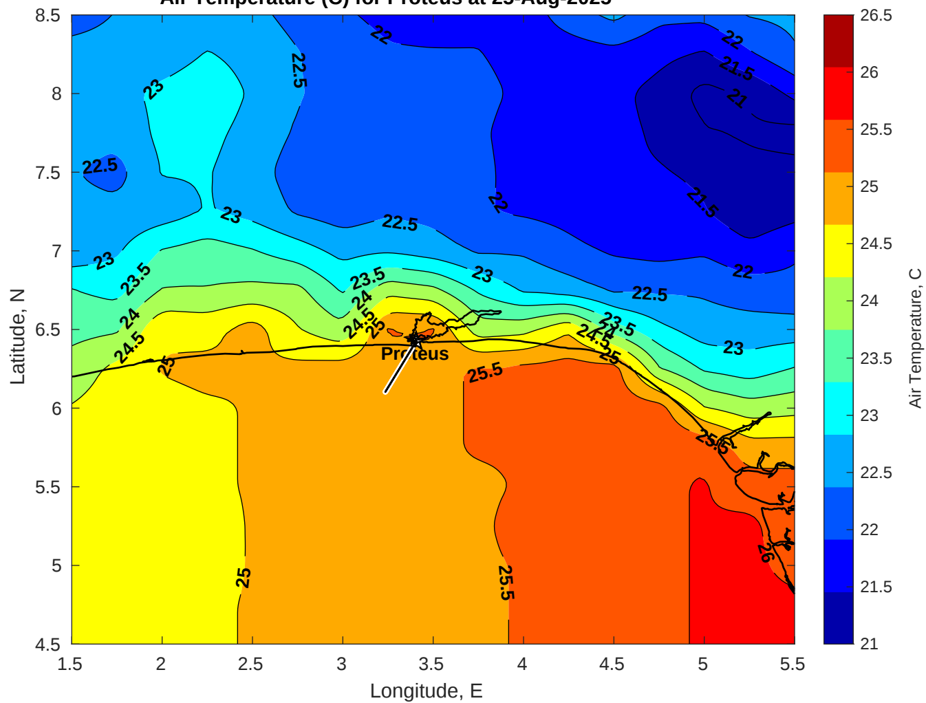
Air Temperature (C) for Proteus at 25-Aug-2025
