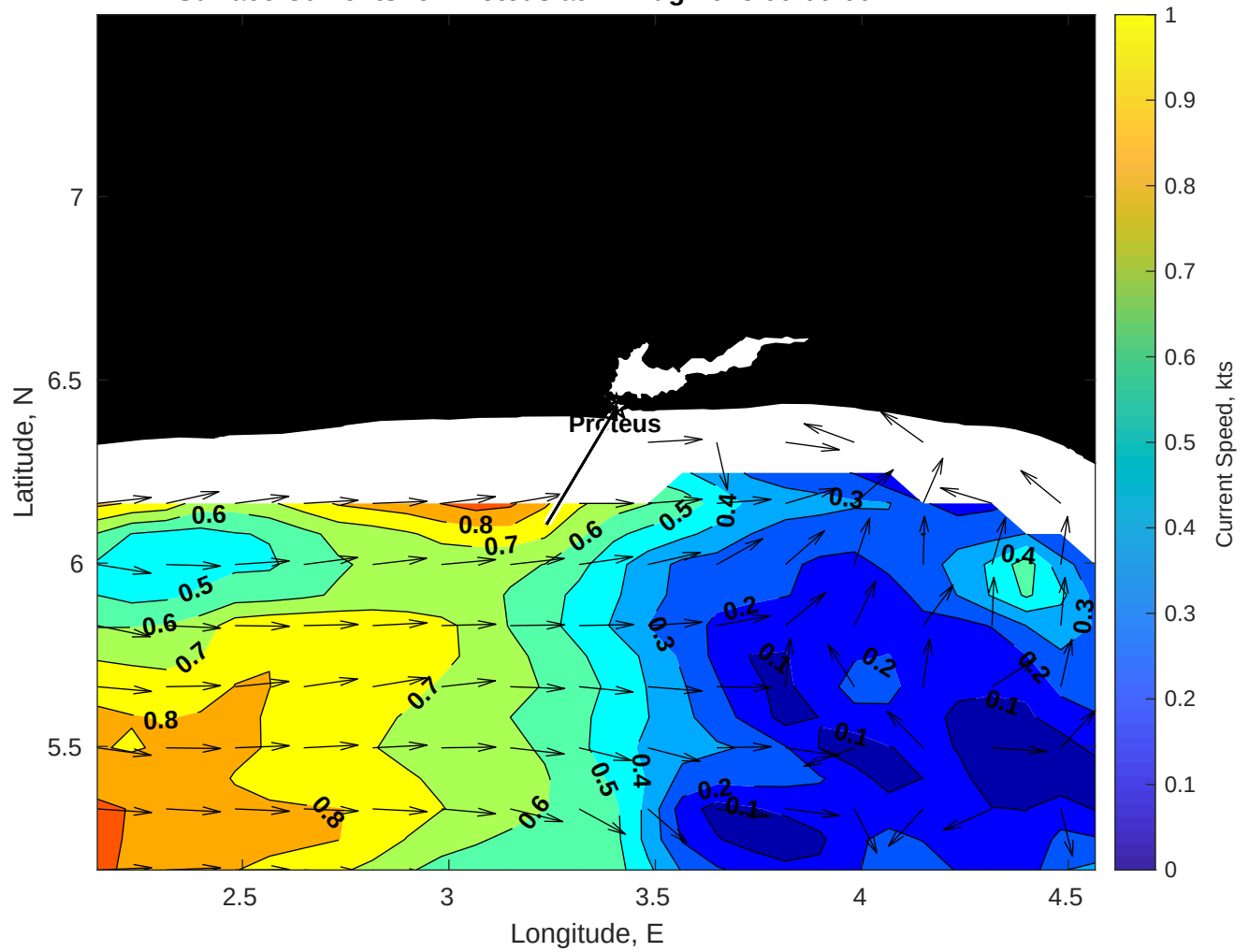
Surface Currents for Proteus at 24-Aug-2025 00:00:00
