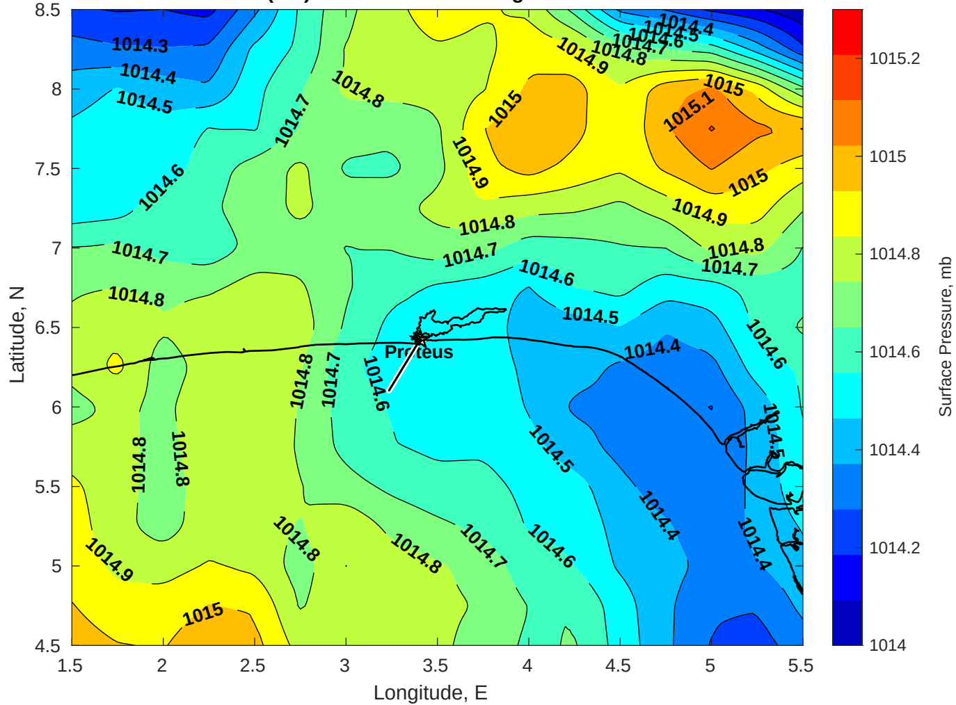
Surface Pressure (mb) for Proteus at 25-Aug-2025 00:00:00
