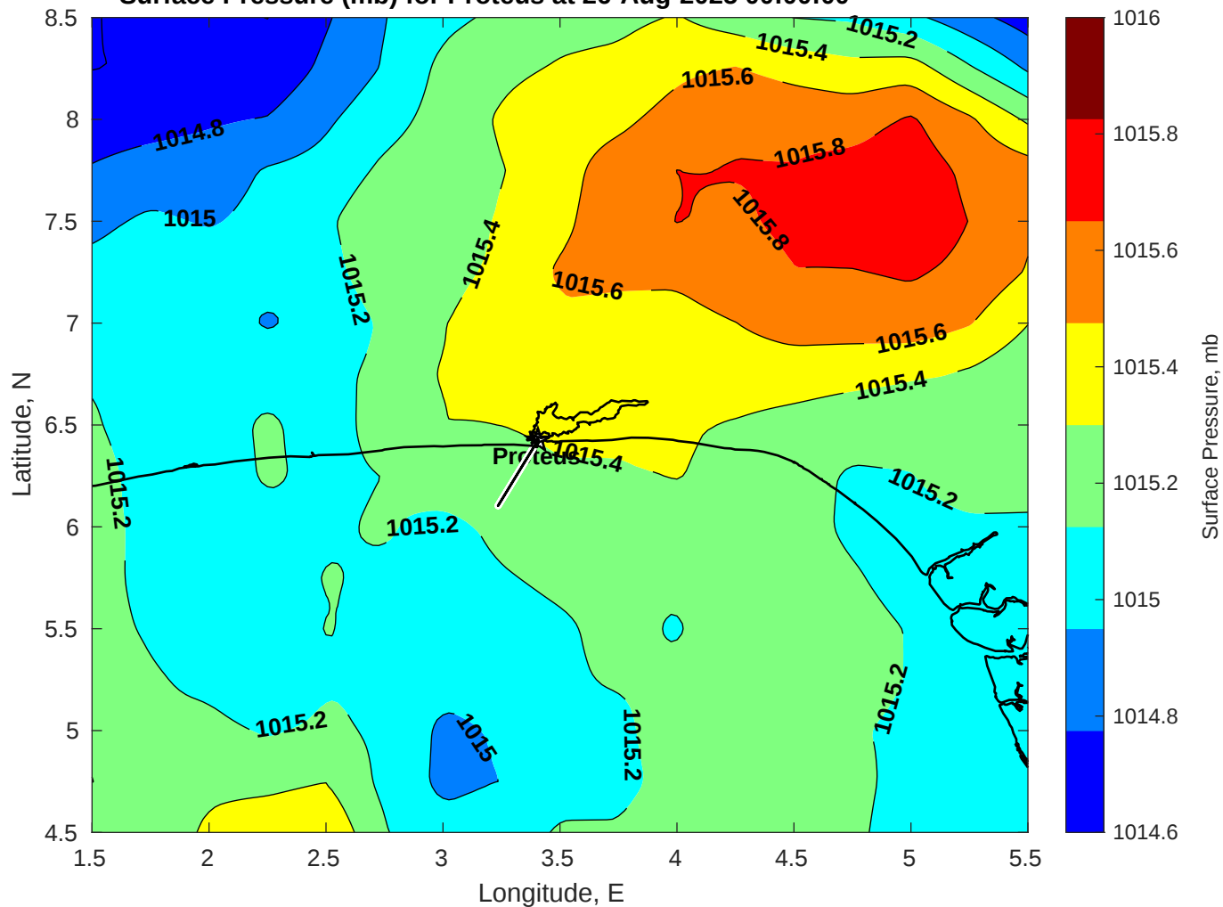
Surface Pressure (mb) for Proteus at 26-Aug-2025 00:00:00
