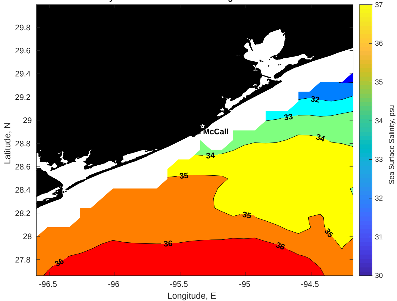
Surface Salinity for Brooks McCall at 25-Aug-2025 00:00:00
