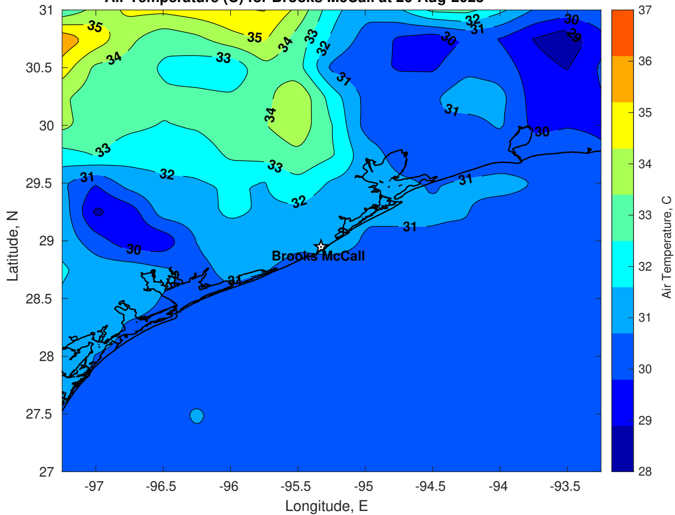
Air Temperature (C) for Brooks McCall at 26-Aug-2025
