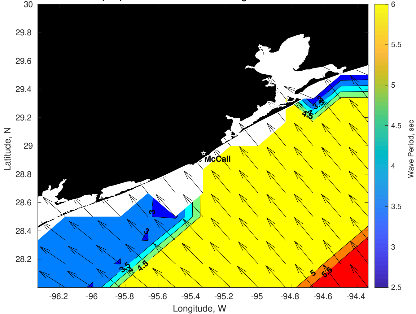
Wave Period (sec) for Brooks McCall at 26-Aug-2025 09:00:00
