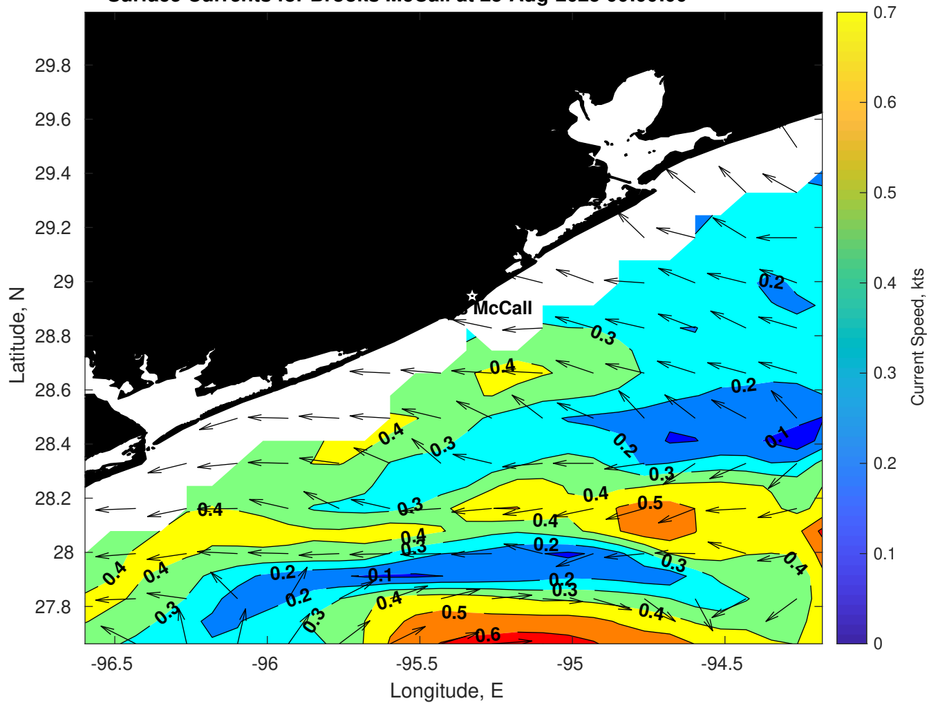
Surface Currents for Brooks McCall at 25-Aug-2025 00:00:00
