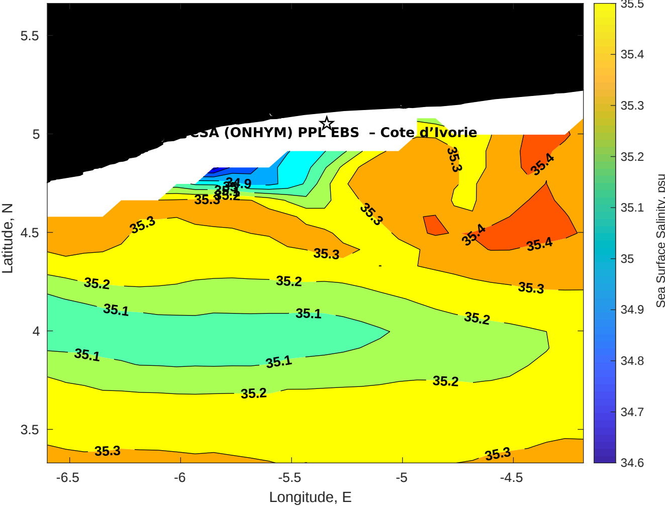
Surface Salinity for CSA (ONHYM) PPL EBS - Cote d'Ivoire at 25-Aug-2025 00:00:00
