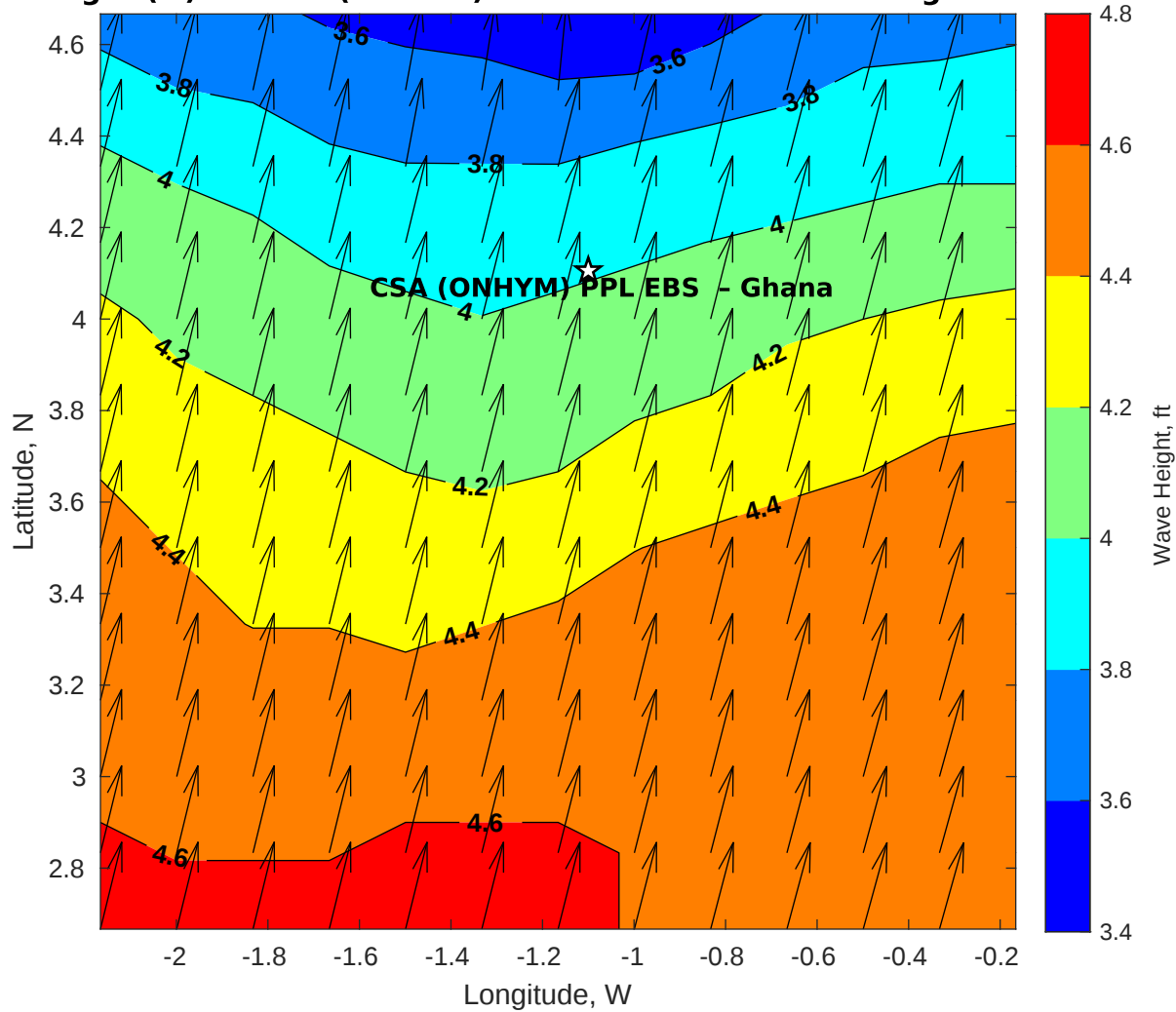
Wave Height (ft) for CSA (ONHYM) PPL EBS - Ghana at 26-Aug-2025 09:00:00
