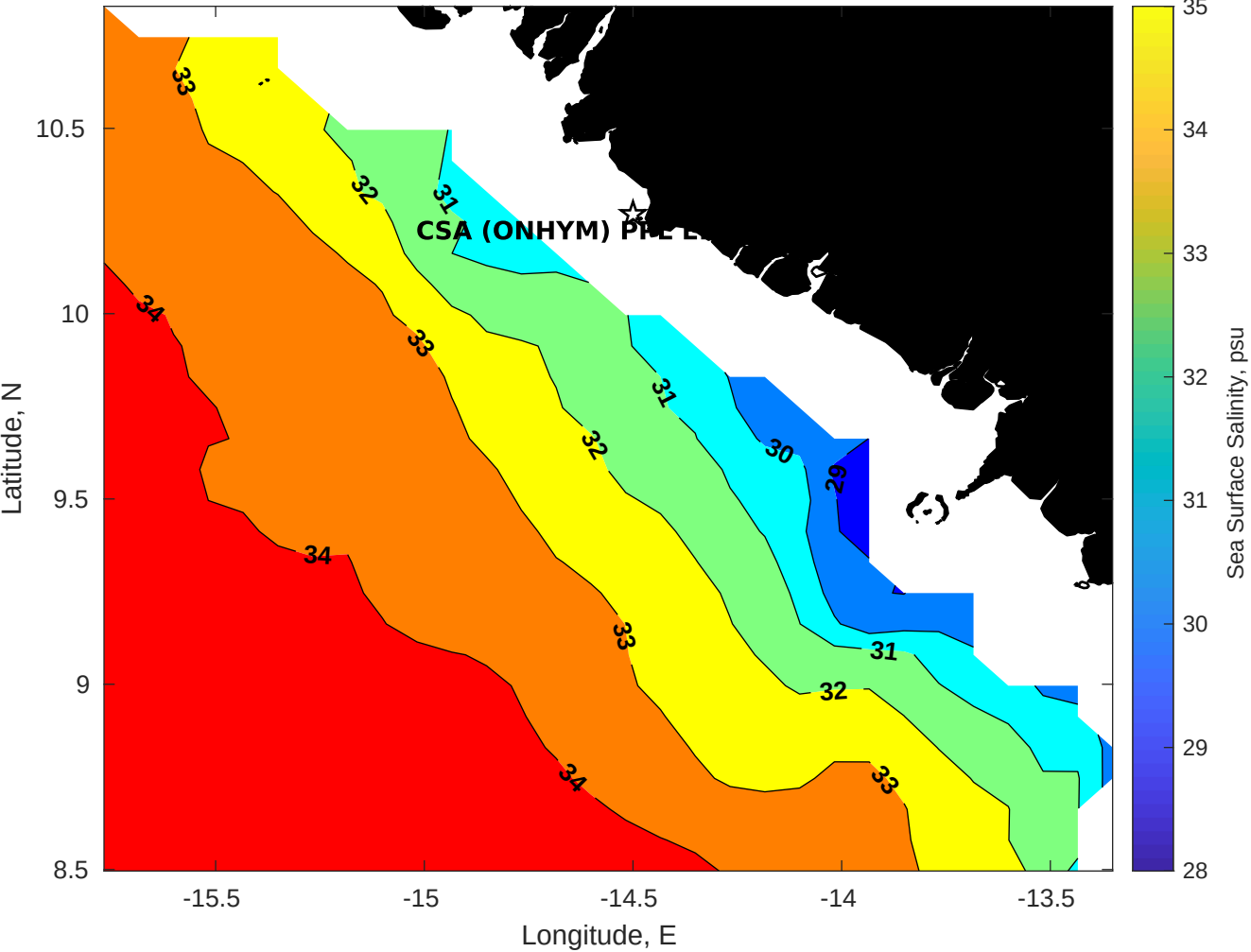
Surface Salinity for CSA (ONHYM) PPL EBS - Guinea at 25-Aug-2025 00:00:00
