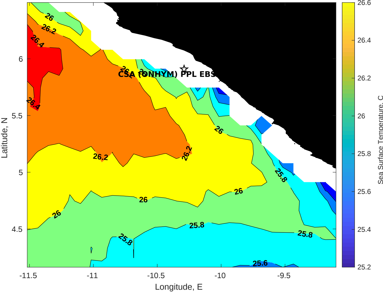
SST for CSA (ONHYM) PPL EBS - Liberia at 25-Aug-2025 00:00:00
