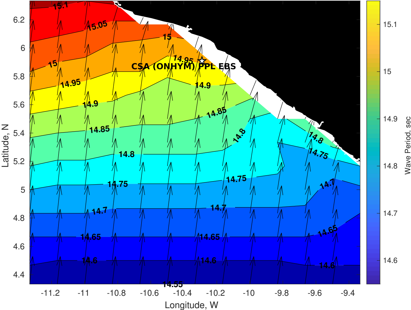
Wave Period (sec) for CSA (ONHYM) PPL EBS - Liberia at 26-Aug-2025 09:00:00
