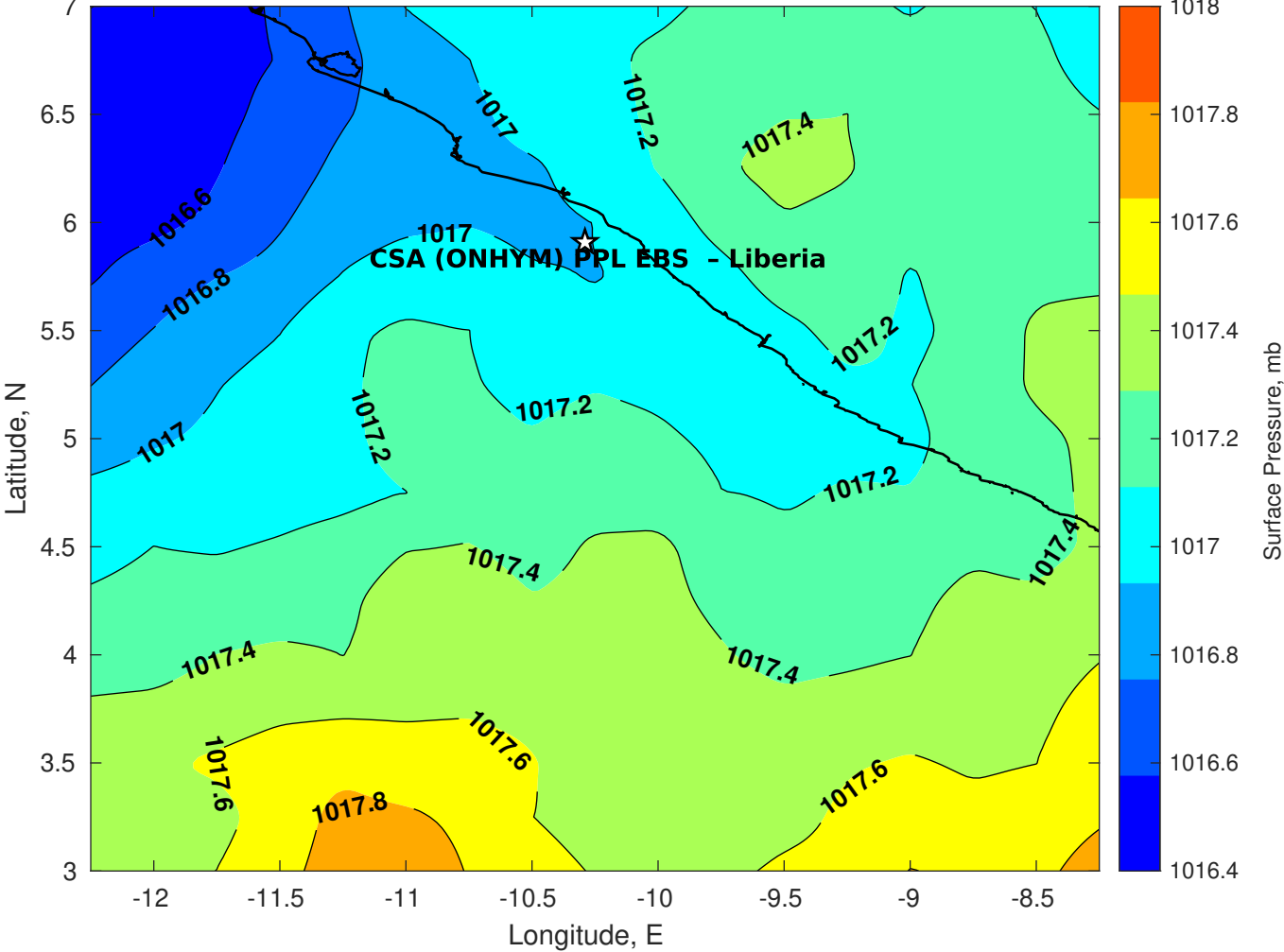
Surface Pressure (mb) for CSA (ONHYM) PPL EBS - Liberia at 27-Aug-2025 00:00:00
