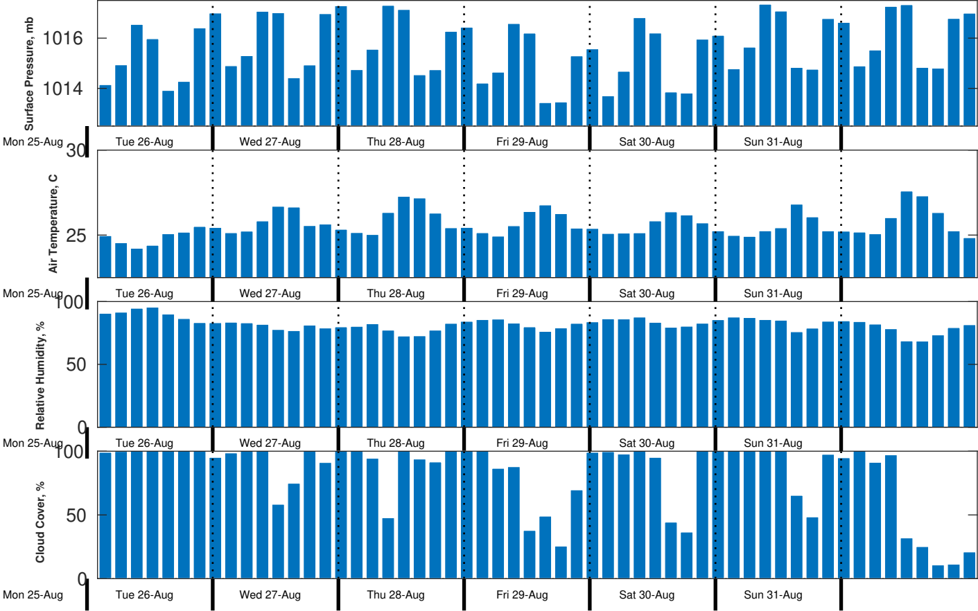
Met Forecast for CSA (ONHYM) PPL EBS - Liberia from 26-Aug-2025 00:00:00 to 02-Sep-2025 00:00:00
