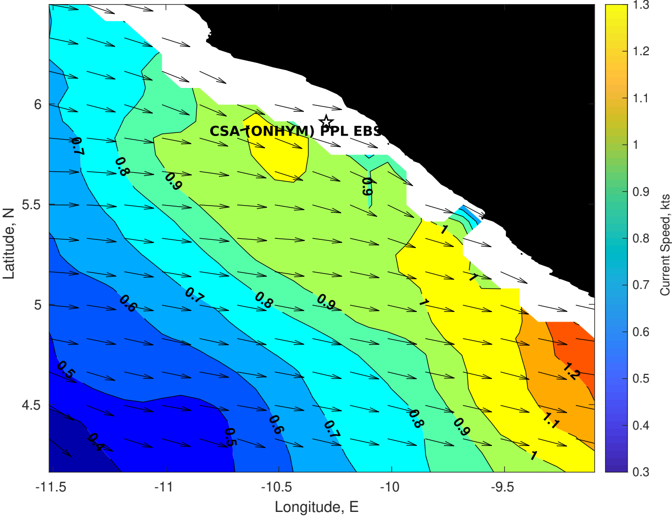
Surface Currents for CSA (ONHYM) PPL EBS - Liberia at 25-Aug-2025 00:00:00
