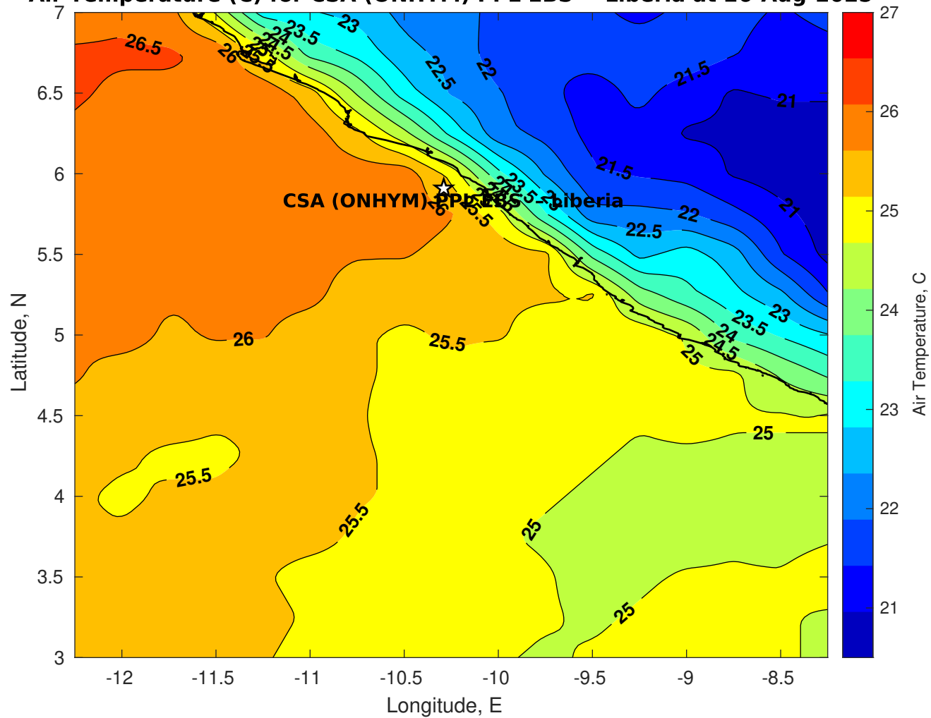
Air Temperature (C) for CSA (ONHYM) PPL EBS - Liberia at 26-Aug-2025
