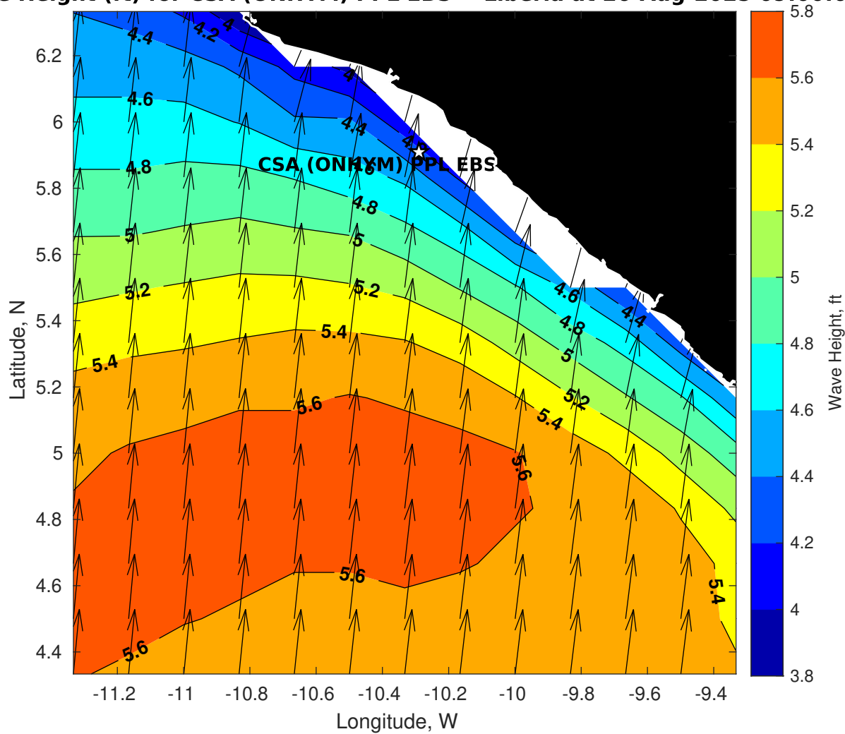
Wave Height (ft) for CSA (ONHYM) PPL EBS - Liberia at 26-Aug-2025 09:00:00
