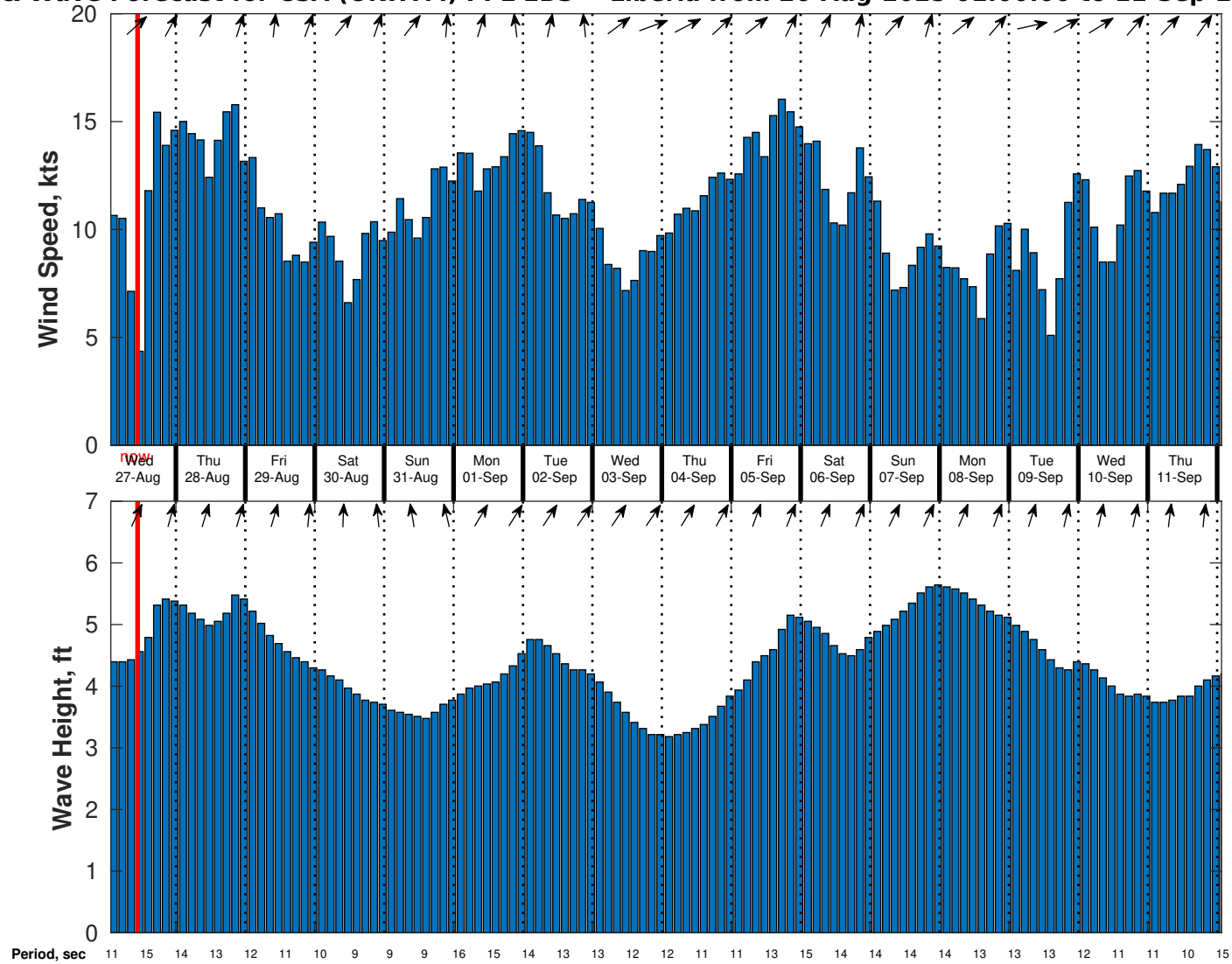
Wind & Wave Forecast for CSA (ONHYM) PPL EBS - Liberia from 26-Aug-2025 01:00:00 to 11-Sep-2025 01:00:00
