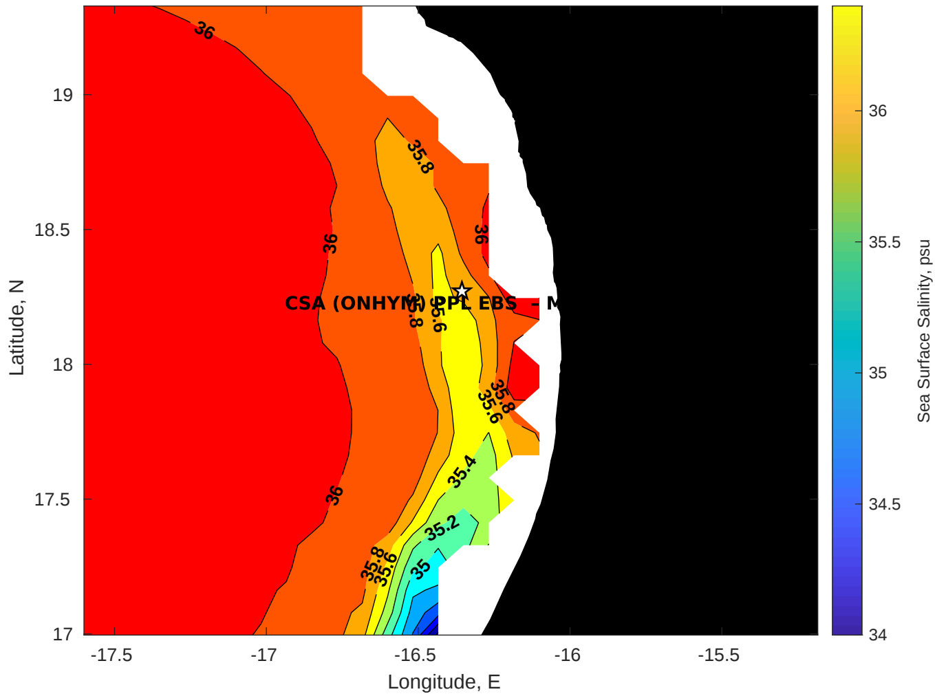
Surface Salinity for CSA (ONHYM) PPL EBS - Mauritania at 25-Aug-2025 00:00:00
