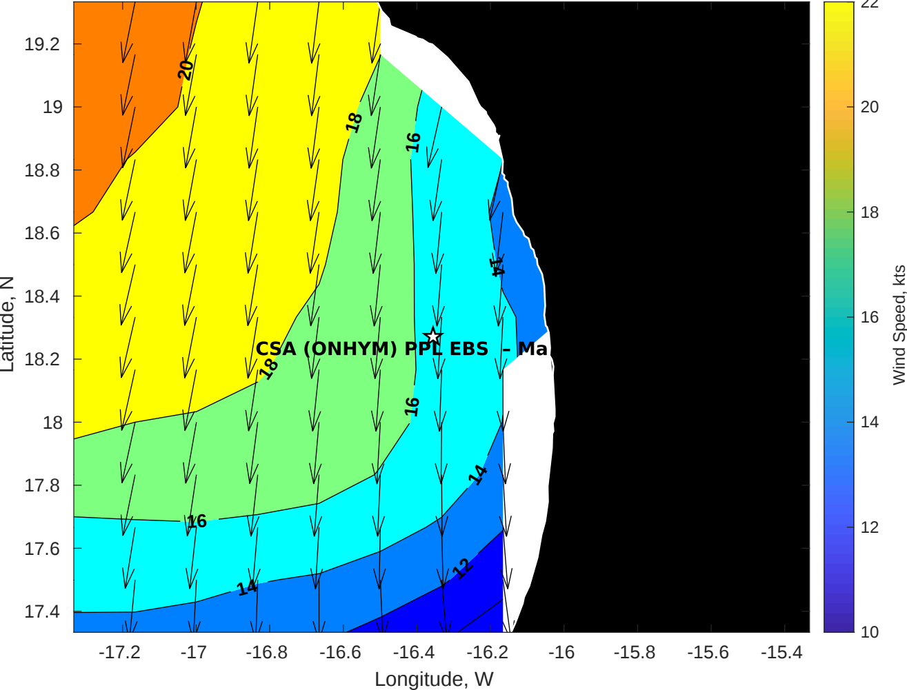
Winds (kts) for CSA (ONHYM) PPL EBS - Mauritania at 26-Aug-2025 09:00:00
