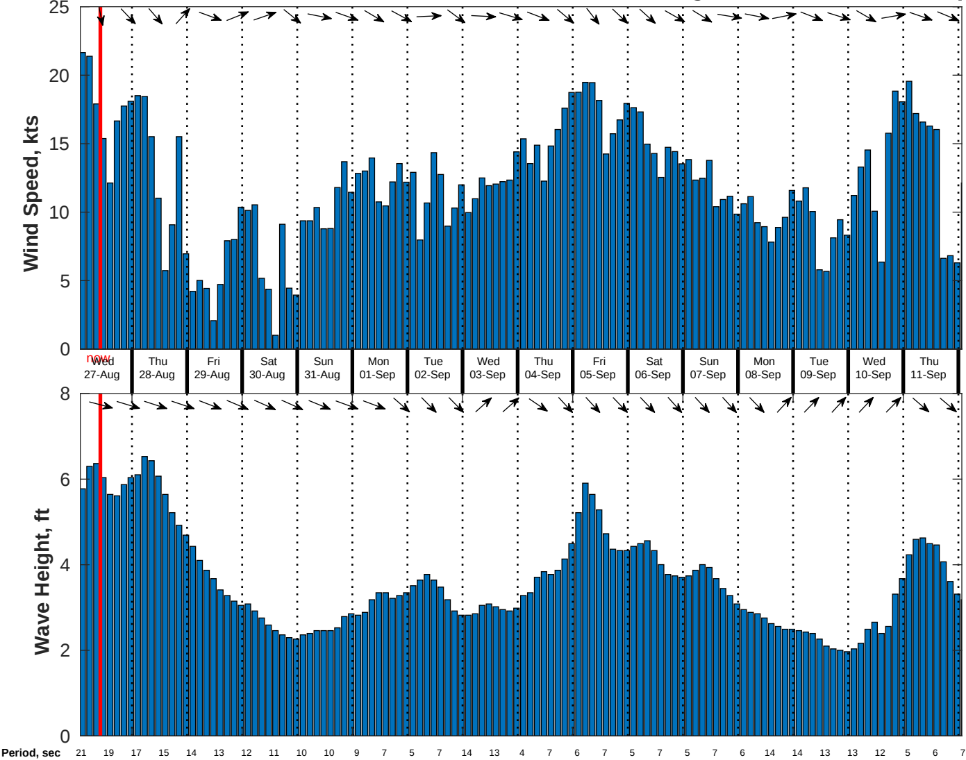
Wind & Wave Forecast for CSA (ONHYM) PPL EBS - Mauritania from 26-Aug-2025 01:00:00 to 11-Sep-2025 01:00:00
