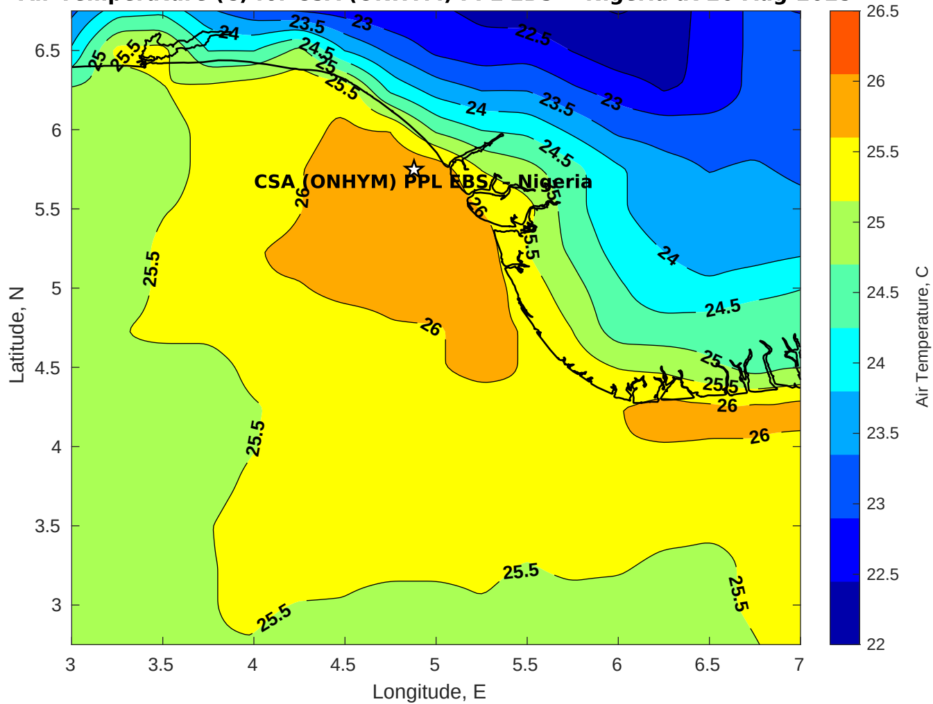
Air Temperature (C) for CSA (ONHYM) PPL EBS - Nigeria at 26-Aug-2025
