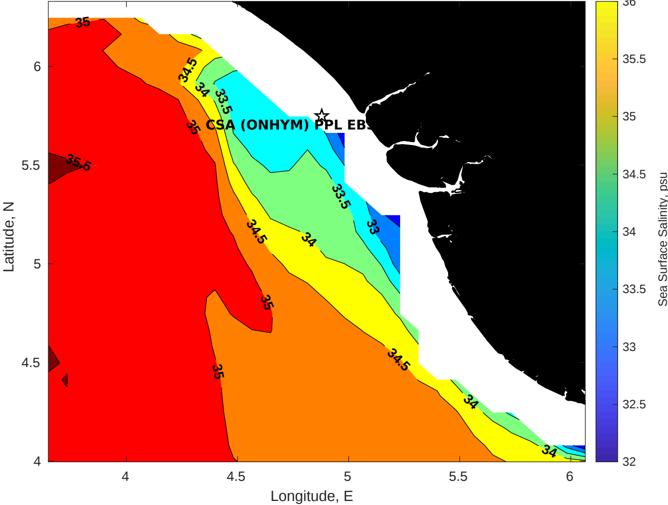
Surface Salinity for CSA (ONHYM) PPL EBS - Nigeria at 25-Aug-2025 00:00:00
