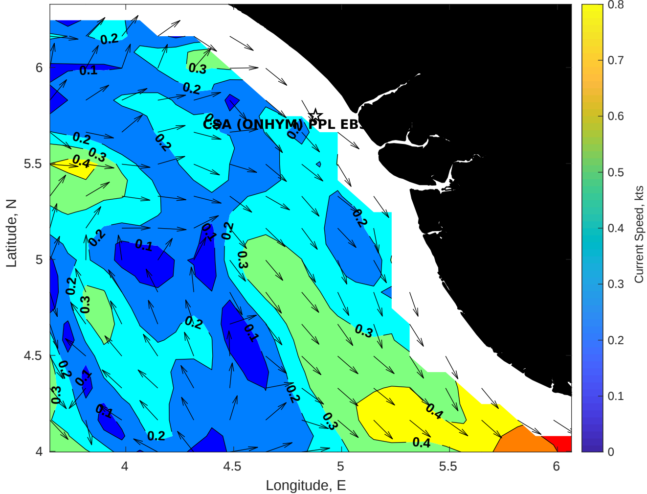
Surface Currents for CSA (ONHYM) PPL EBS - Nigeria at 25-Aug-2025 00:00:00
