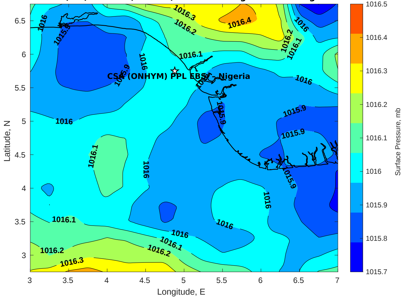
Surface Pressure (mb) for CSA (ONHYM) PPL EBS - Nigeria at 28-Aug-2025 00:00:00
