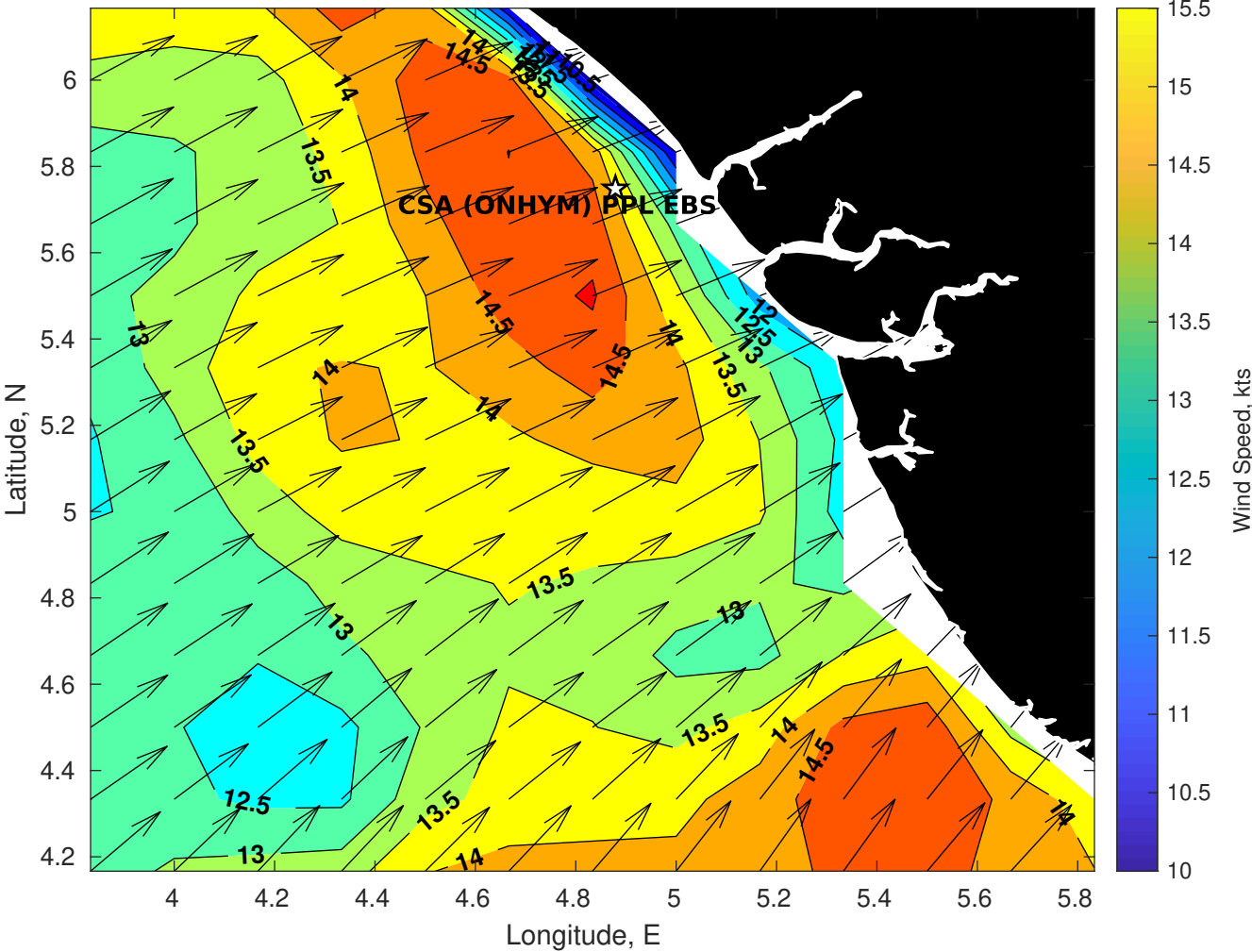
Winds (kts) for CSA (ONHYM) PPL EBS - Nigeria at 26-Aug-2025 09:00:00
