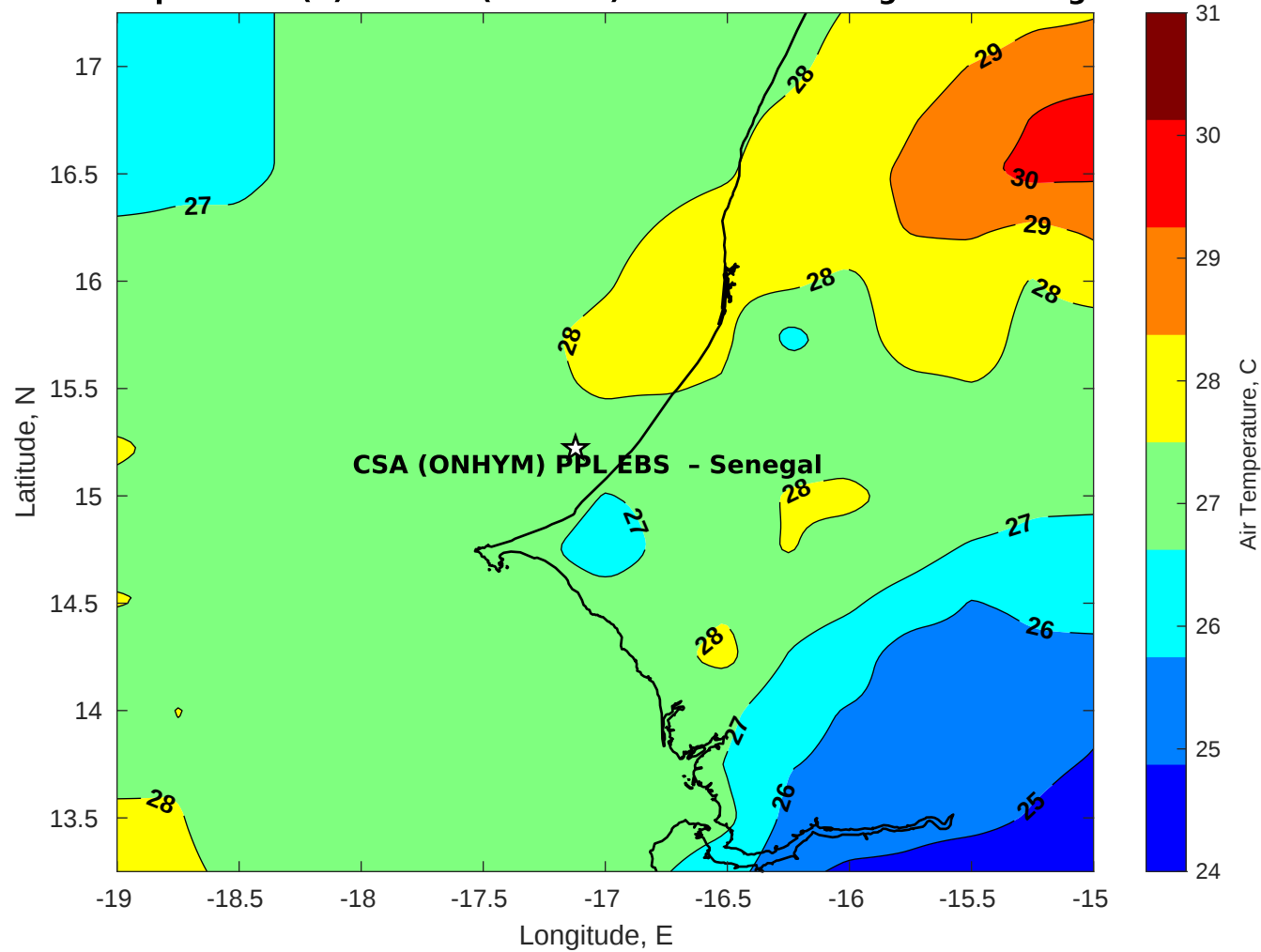
Air Temperature (C) for CSA (ONHYM) PPL EBS - Senegal at 26-Aug-2025
