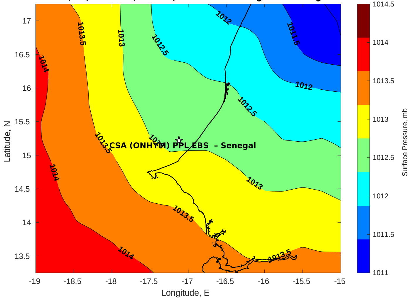
Surface Pressure (mb) for CSA (ONHYM) PPL EBS - Senegal at 27-Aug-2025 00:00:00
