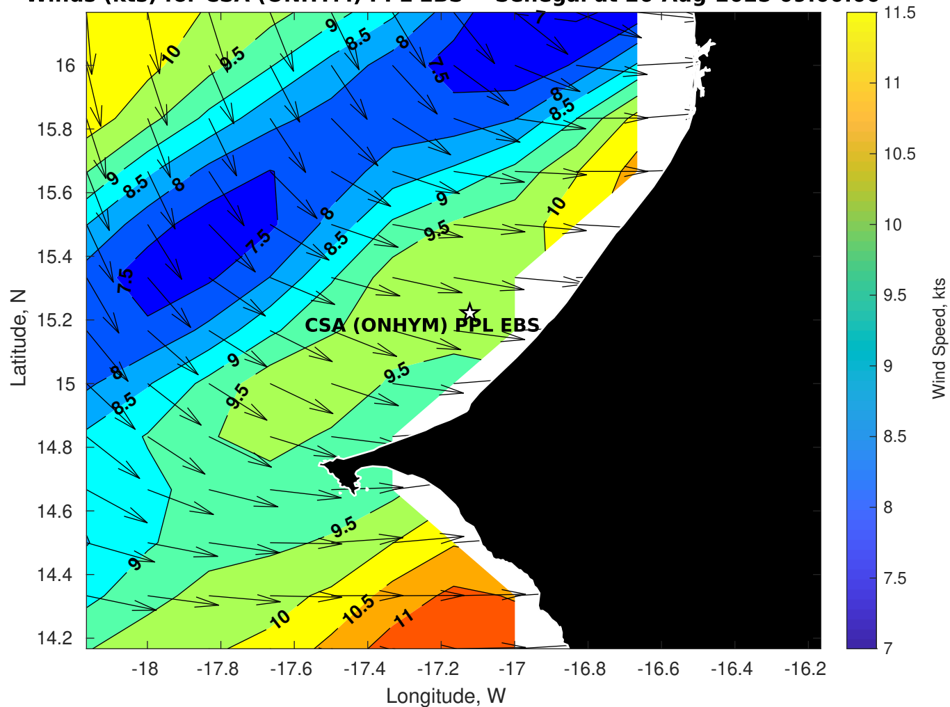
Winds (kts) for CSA (ONHYM) PPL EBS - Senegal at 26-Aug-2025 09:00:00
