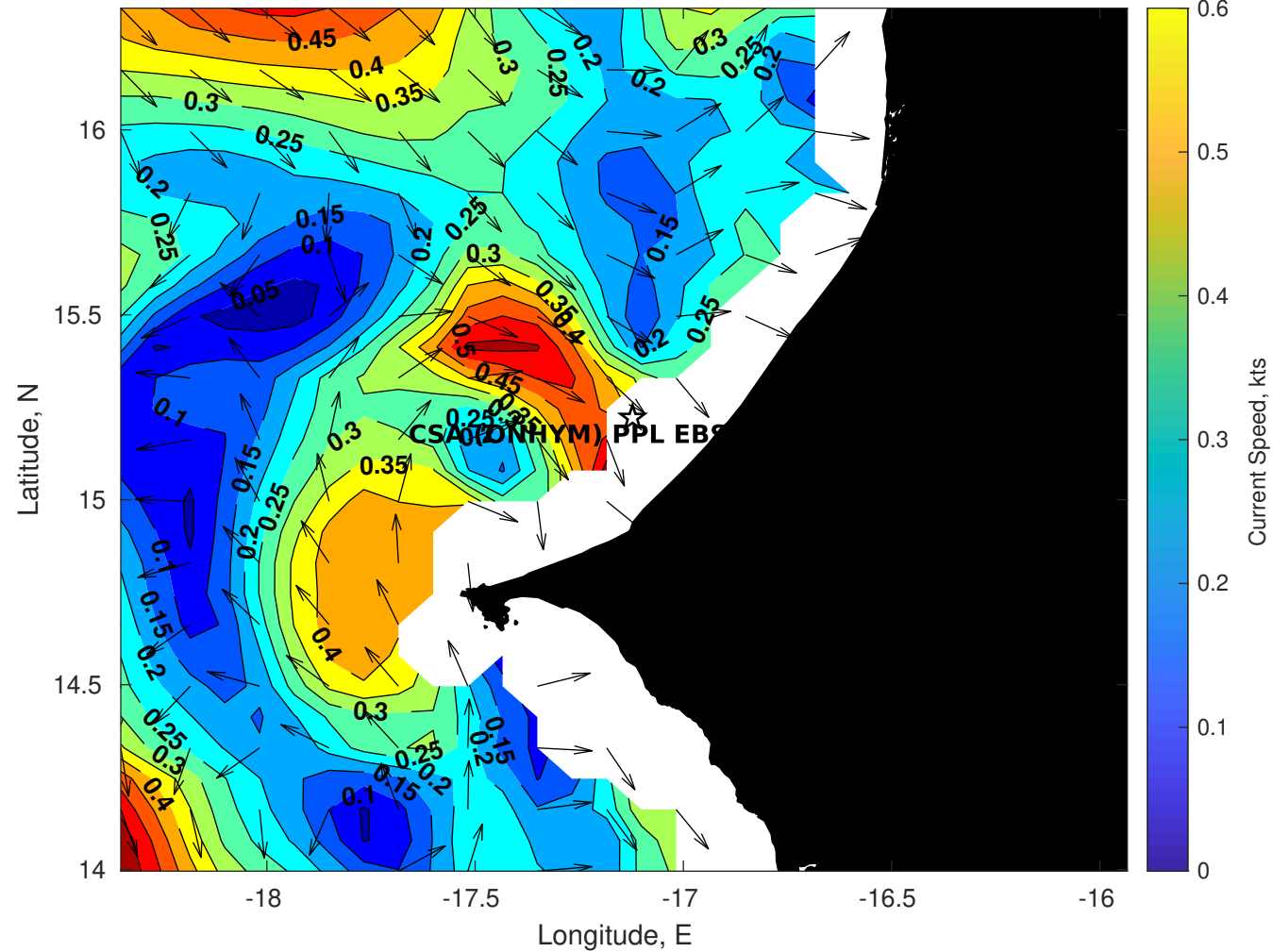
Surface Currents for CSA (ONHYM) PPL EBS - Senegal at 25-Aug-2025 00:00:00
