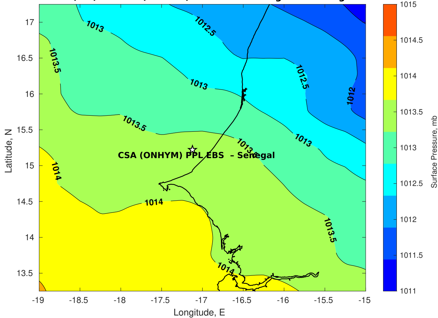
Surface Pressure (mb) for CSA (ONHYM) PPL EBS - Senegal at 26-Aug-2025 00:00:00
