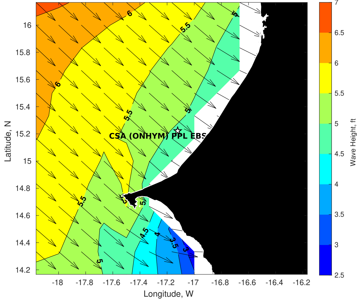
Wave Height (ft) for CSA (ONHYM) PPL EBS - Senegal at 26-Aug-2025 09:00:00
