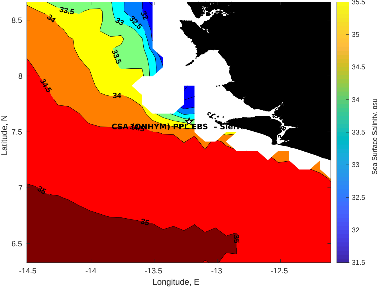
Surface Salinity for CSA (ONHYM) PPL EBS - Sierra Leone at 25-Aug-2025 00:00:00
