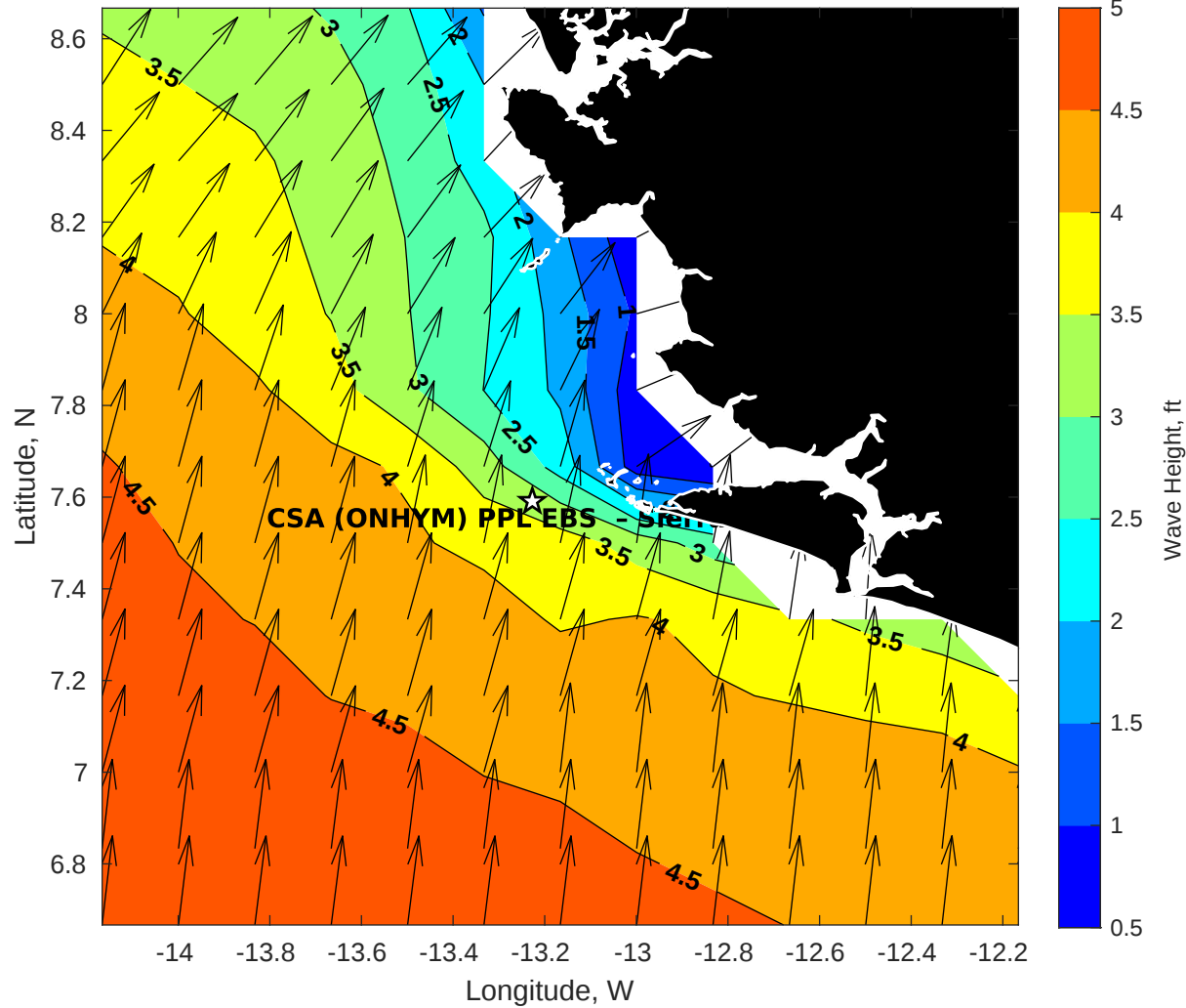
Wave Height (ft) for CSA (ONHYM) PPL EBS - Sierra Leone at 26-Aug-2025 09:00:00
