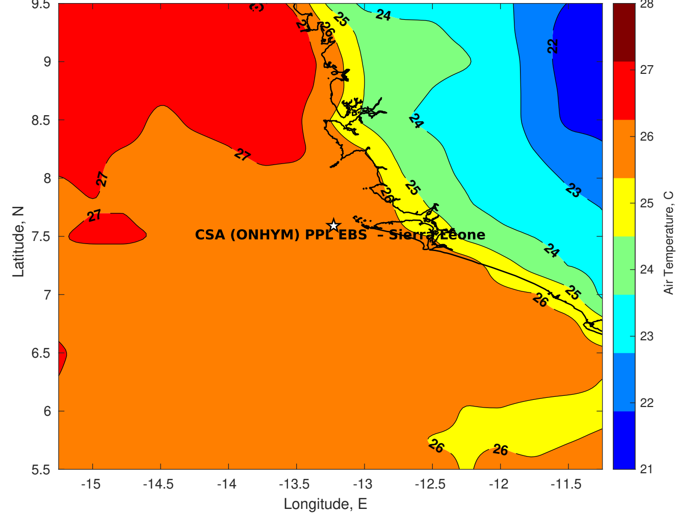
Air Temperature (C) for CSA (ONHYM) PPL EBS - Sierra Leone at 26-Aug-2025
