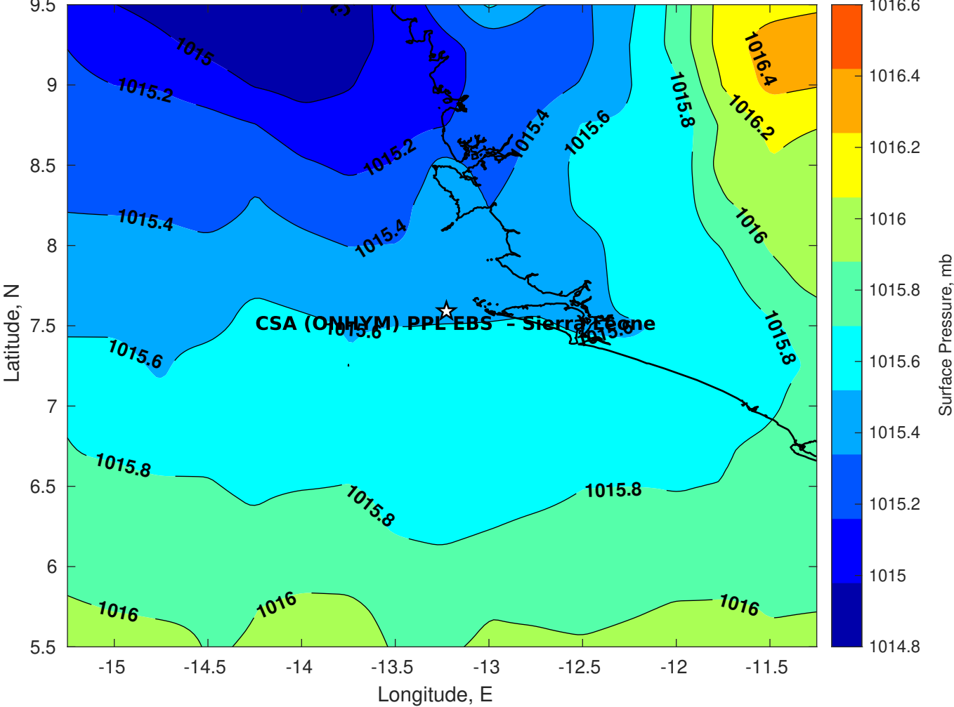
Surface Pressure (mb) for CSA (ONHYM) PPL EBS - Sierra Leone at 26-Aug-2025 00:00:00
