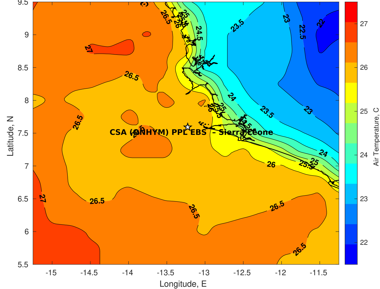
Air Temperature (C) for CSA (ONHYM) PPL EBS - Sierra Leone at 26-Aug-2025
