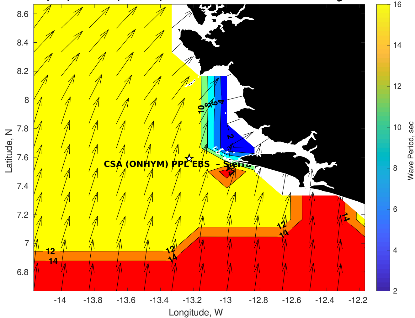
Wave Period (sec) for CSA (ONHYM) PPL EBS - Sierra Leone at 26-Aug-2025 09:00:00
