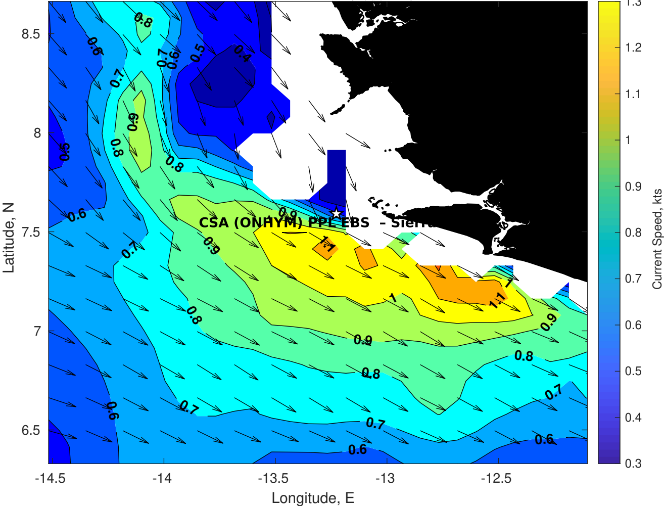
Surface Currents for CSA (ONHYM) PPL EBS - Sierra Leone at 25-Aug-2025 00:00:00
