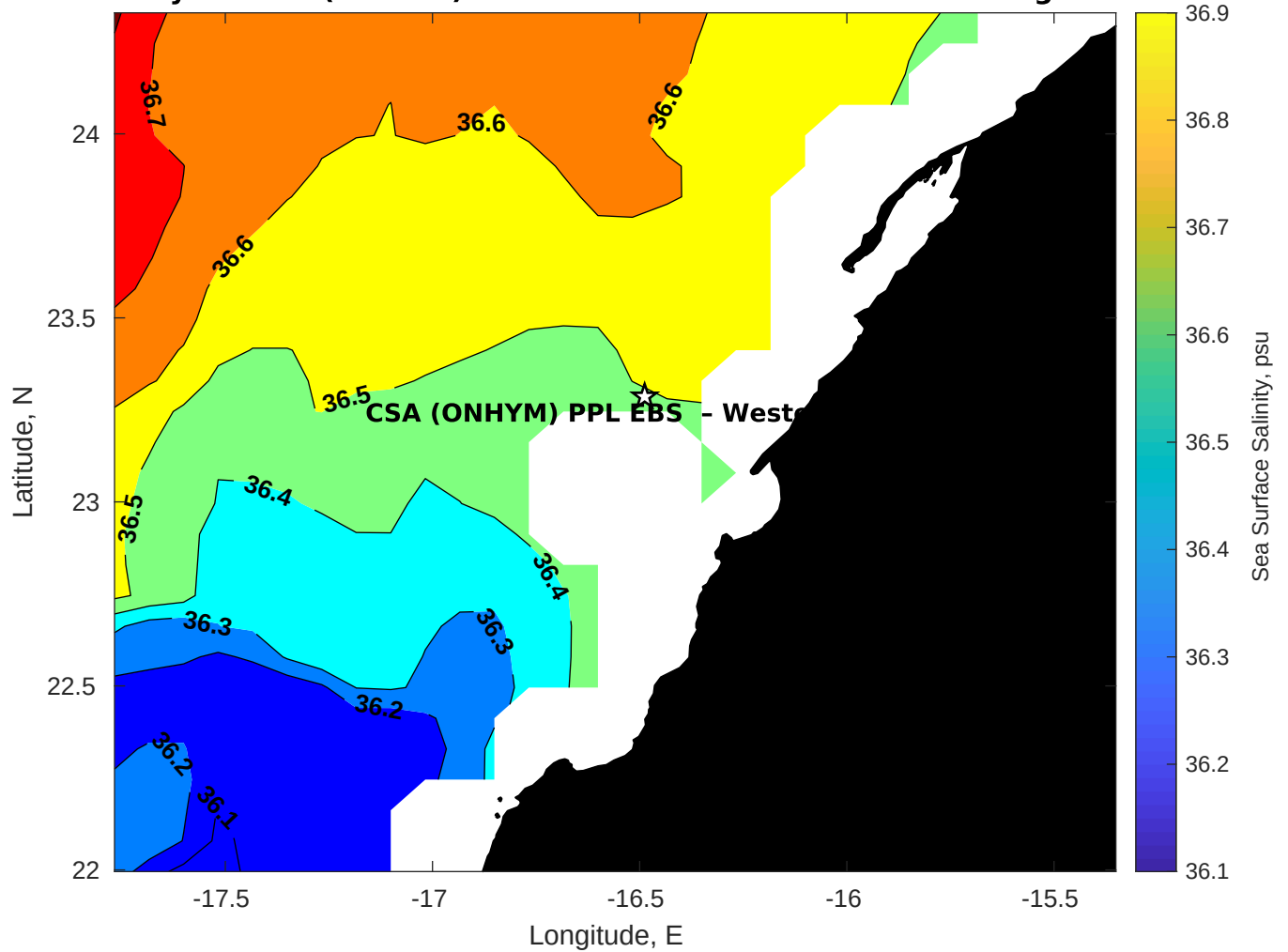
Surface Salinity for CSA (ONHYM) PPL EBS - Western Sahara at 25-Aug-2025 00:00:00
