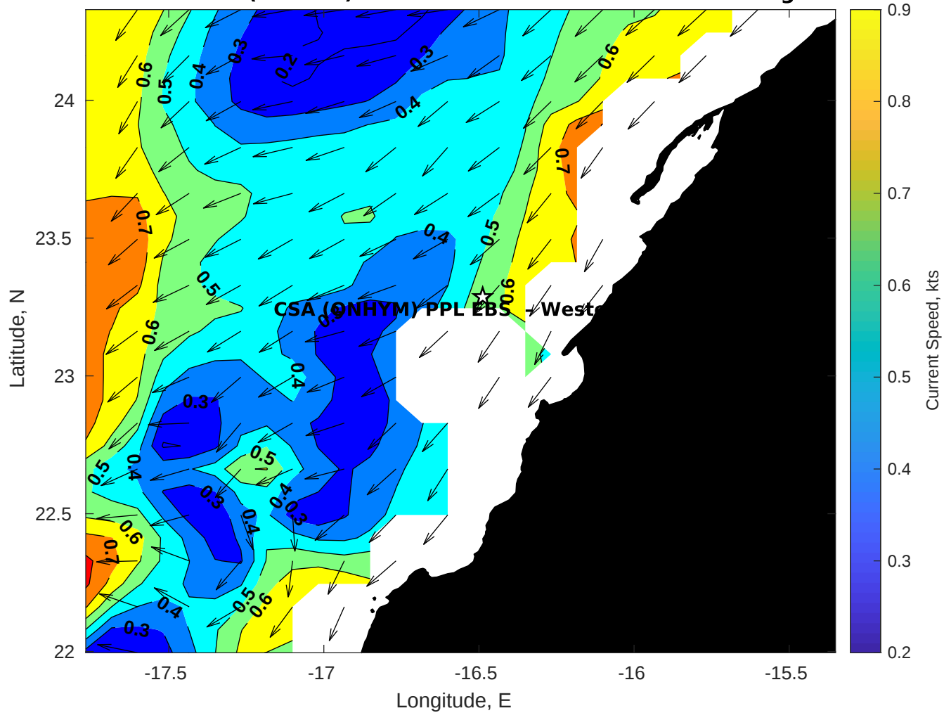
Surface Currents for CSA (ONHYM) PPL EBS - Western Sahara at 25-Aug-2025 00:00:00
