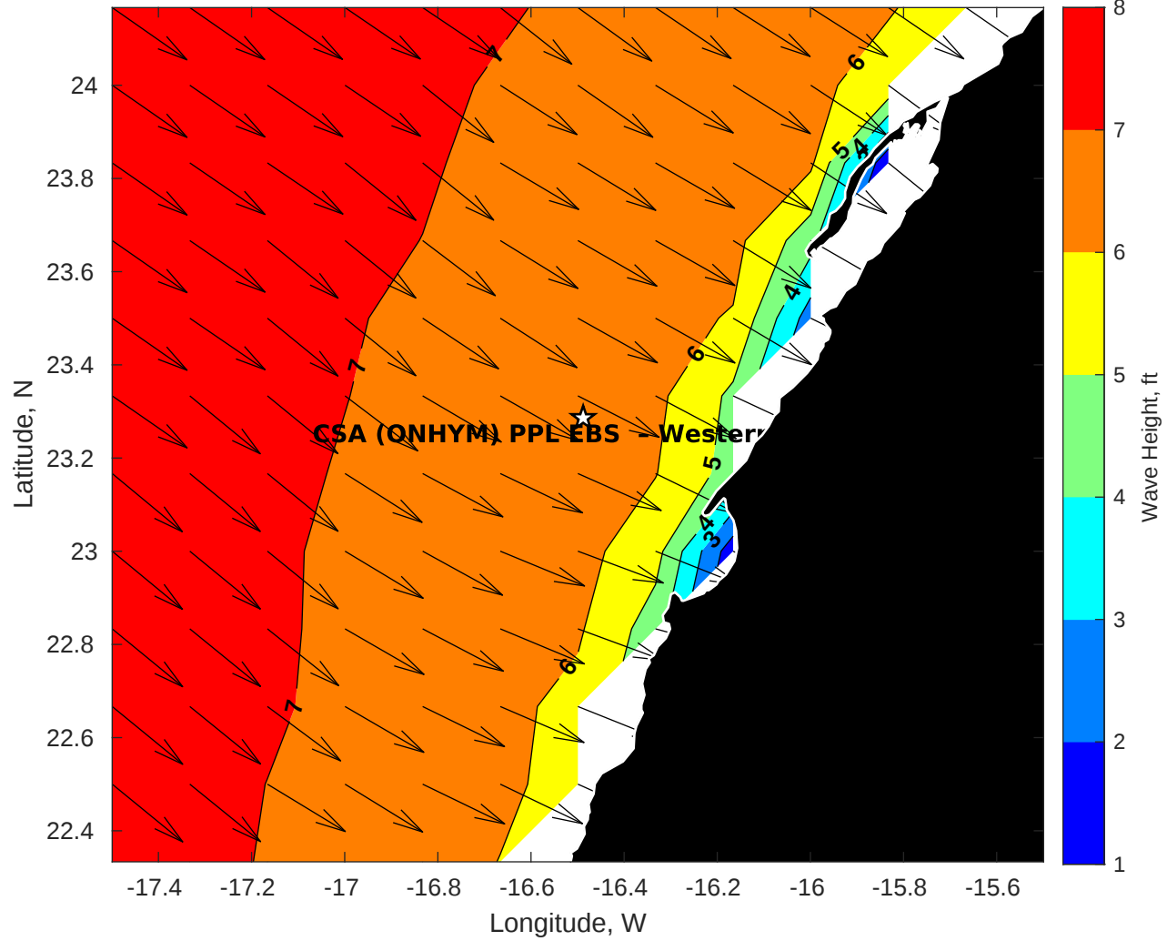
Wave Height (ft) for CSA (ONHYM) PPL EBS - Western Sahara at 26-Aug-2025 09:00:00
