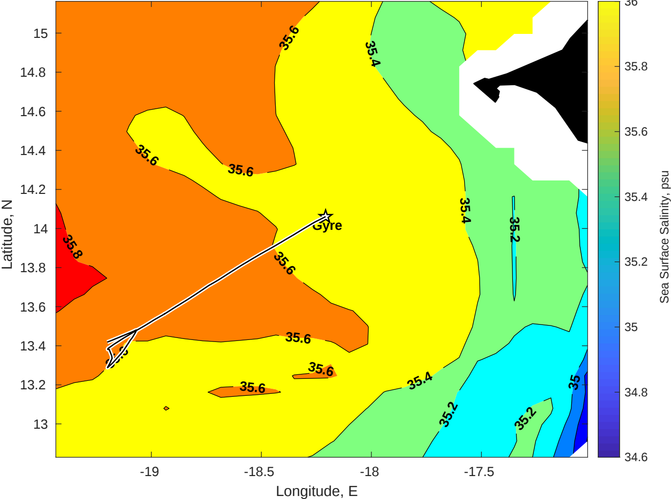
Surface Salinity for Gyre at 25-Aug-2025 00:00:00
