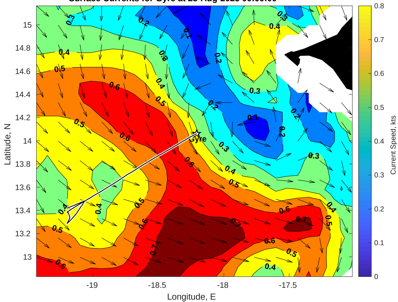
Surface Currents for Gyre at 25-Aug-2025 00:00:00
