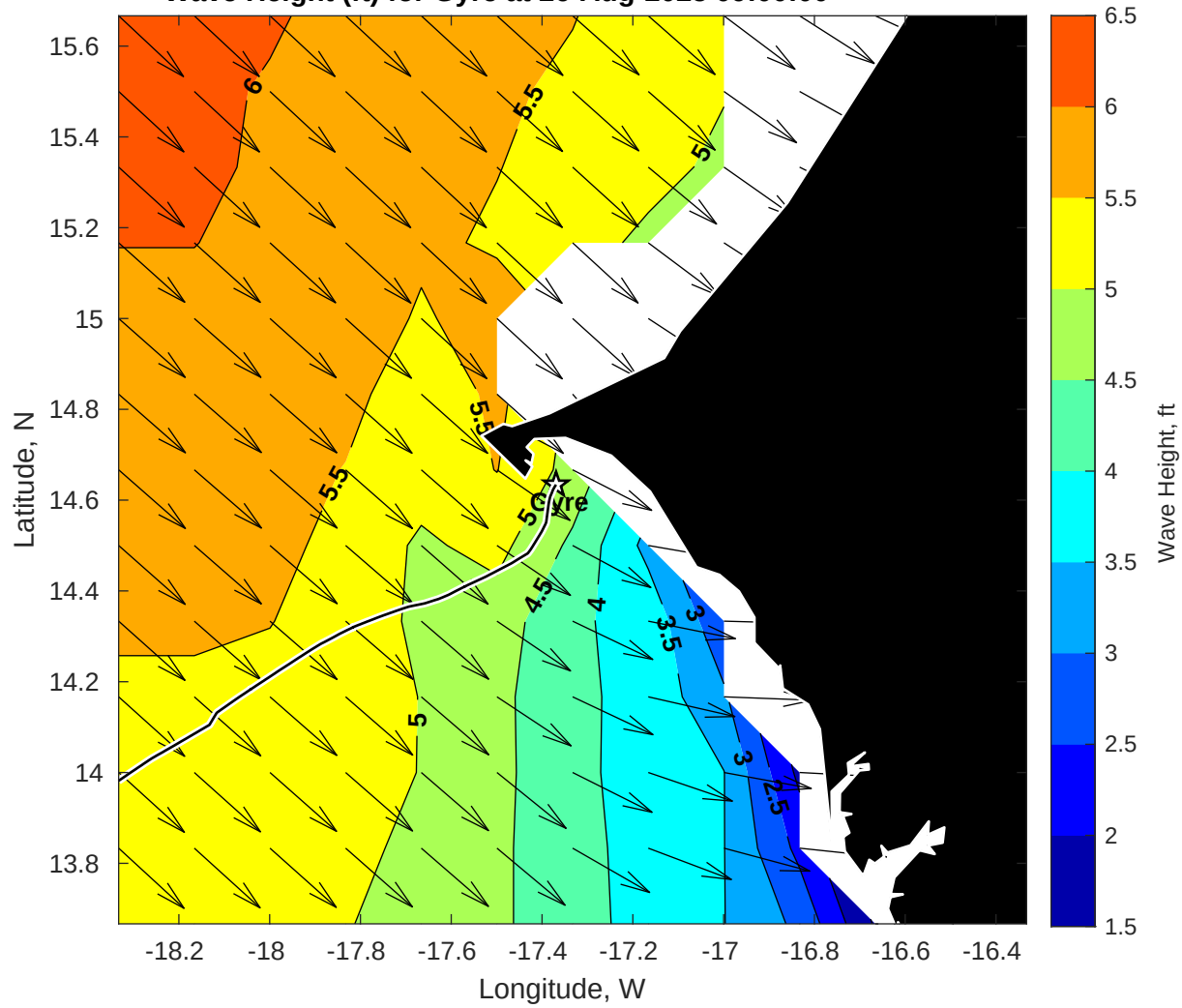
Wave Height (ft) for Gyre at 26-Aug-2025 09:00:00
