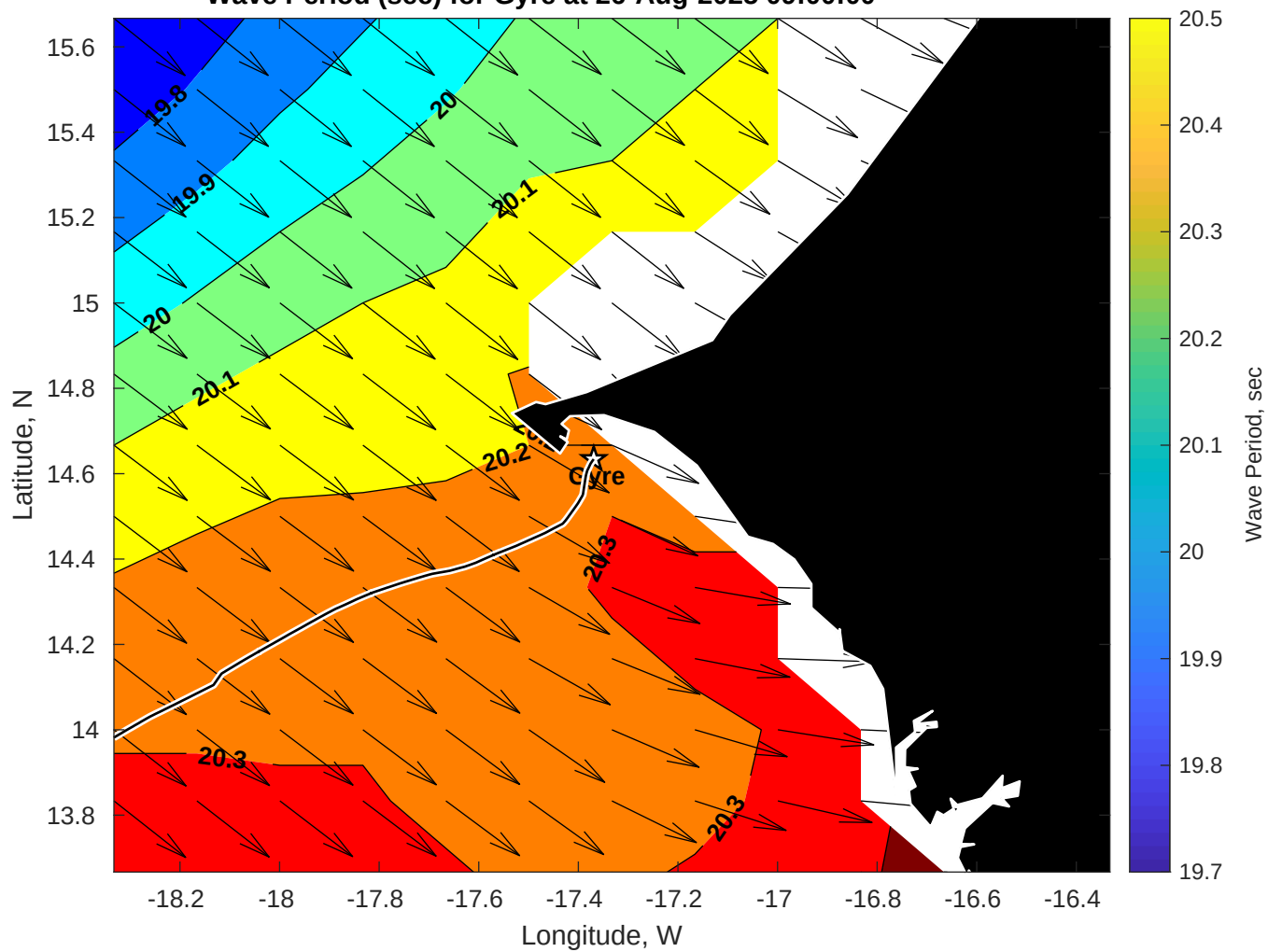
Wave Period (sec) for Gyre at 26-Aug-2025 09:00:00
