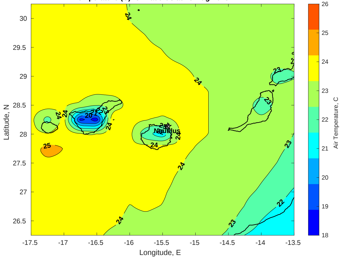
Air Temperature (C) for Nautilus at 26-Aug-2025
