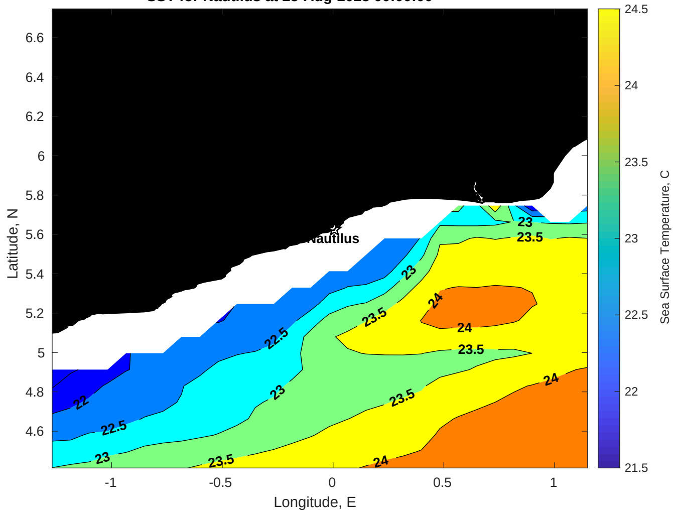
SST for Nautilus at 25-Aug-2025 00:00:00
