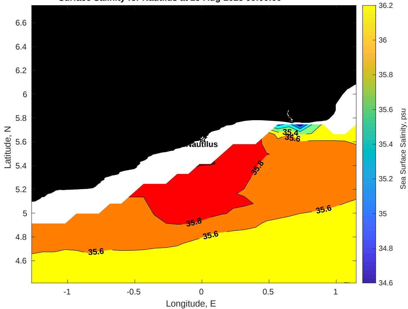
Surface Salinity for Nautilus at 25-Aug-2025 00:00:00
