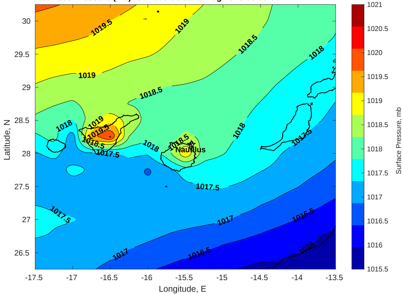
Surface Pressure (mb) for Nautilus at 28-Aug-2025 00:00:00
