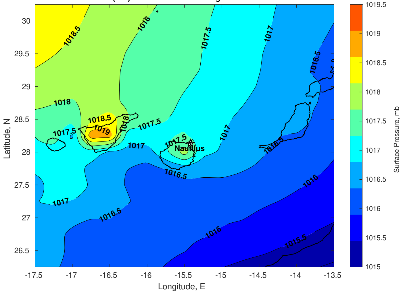
Surface Pressure (mb) for Nautilus at 27-Aug-2025 00:00:00
