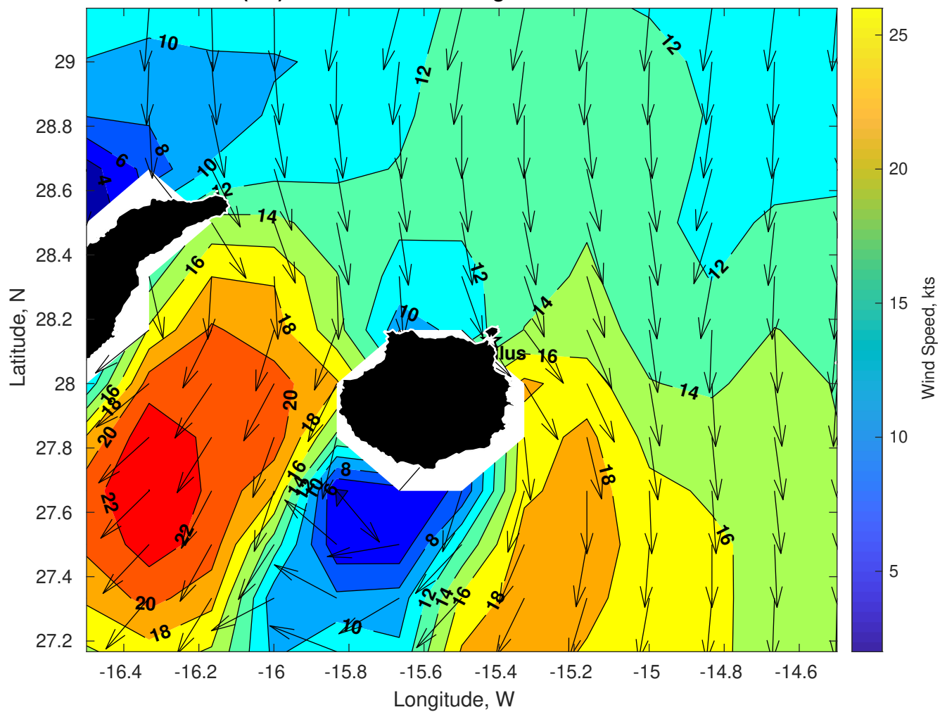
Winds (kts) for Nautilus at 26-Aug-2025 09:00:00
