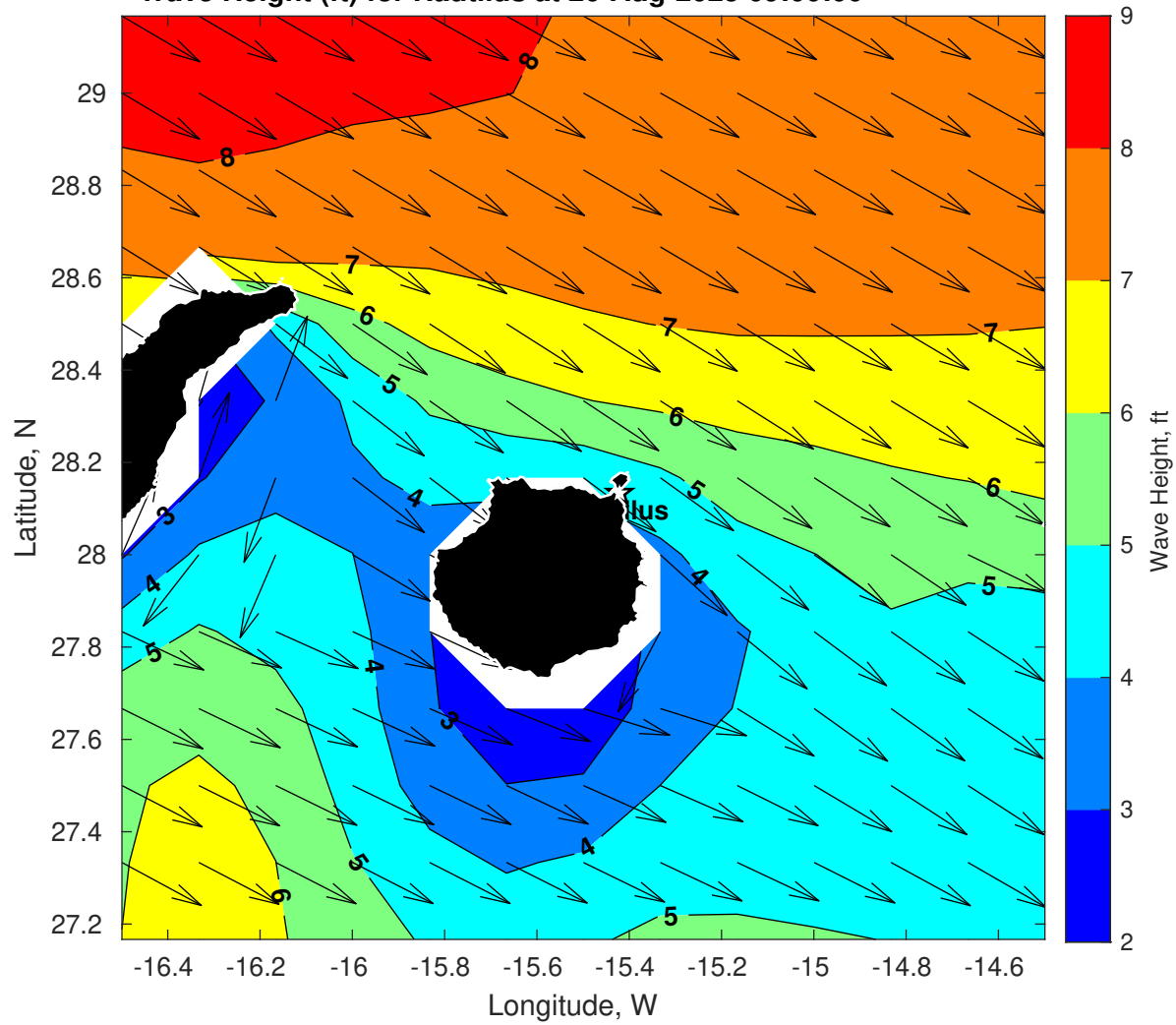
Wave Height (ft) for Nautilus at 26-Aug-2025 09:00:00
