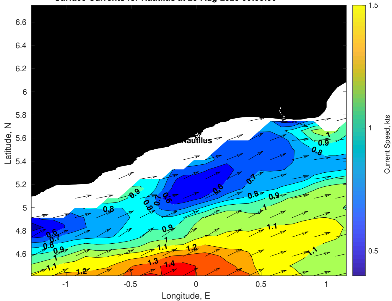
Surface Currents for Nautilus at 25-Aug-2025 00:00:00
