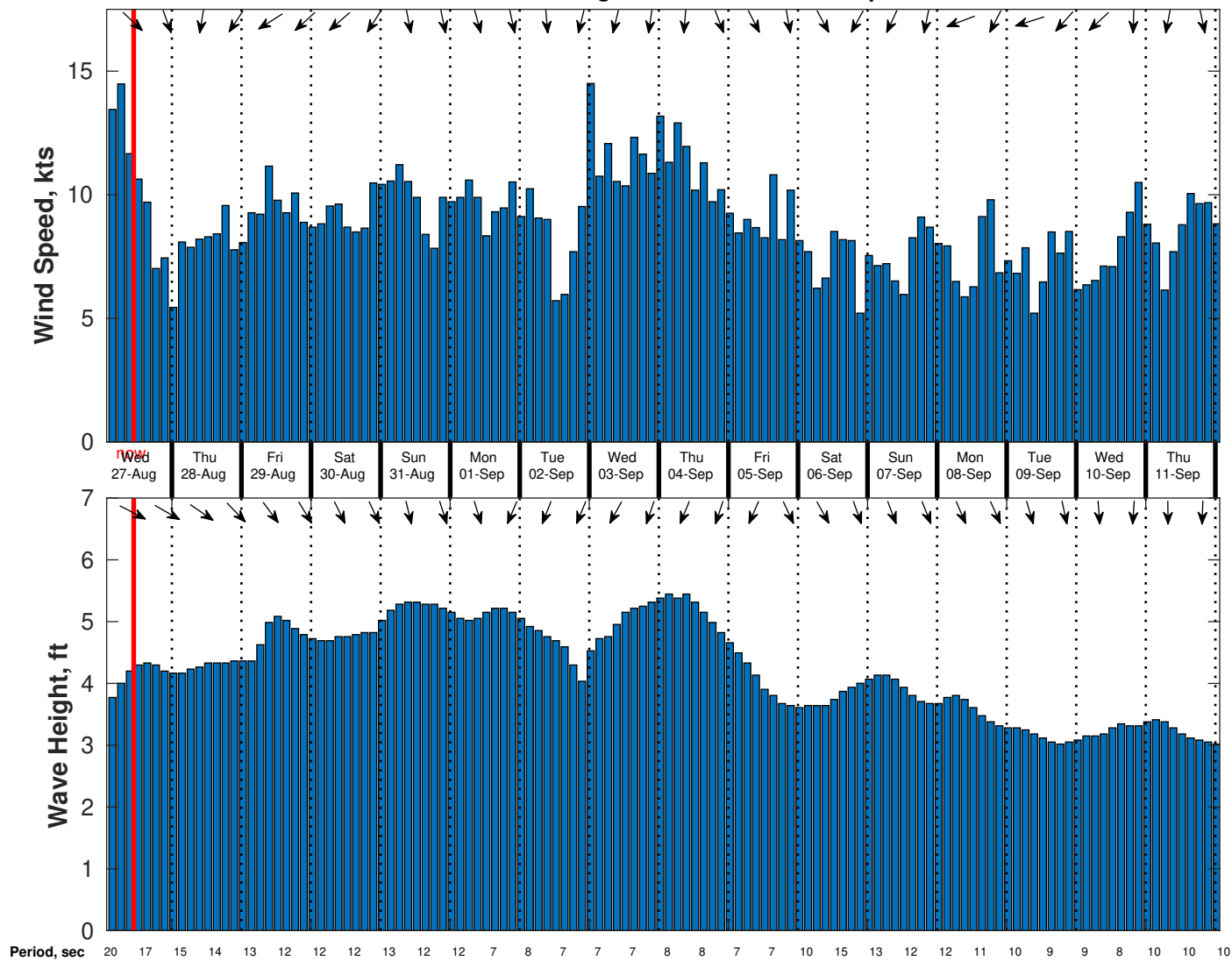
Wind & Wave Forecast for Nautilus from 26-Aug-2025 02:00:00 to 11-Sep-2025 02:00:00
