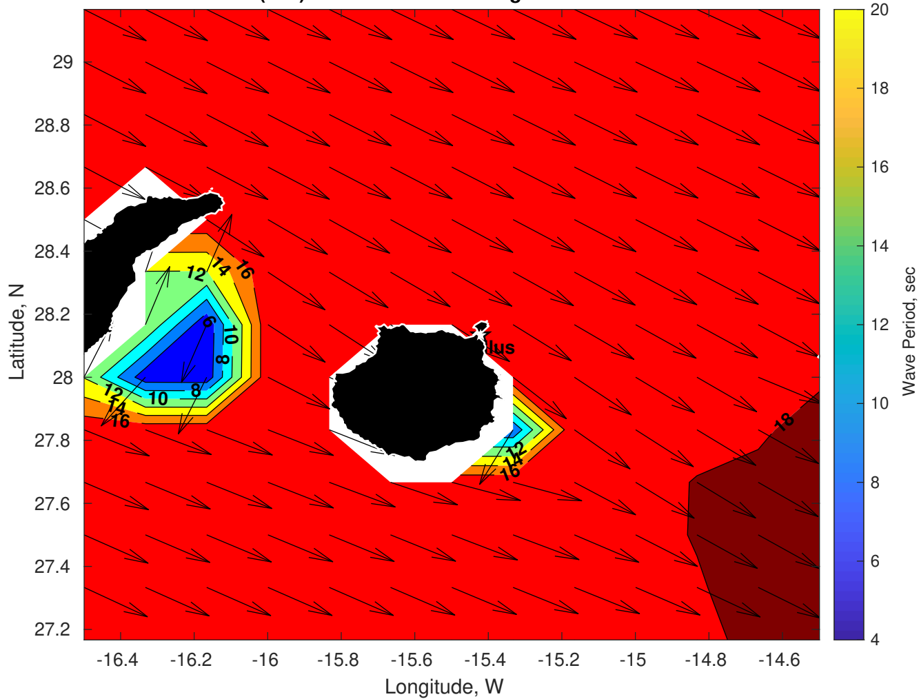
Wave Period (sec) for Nautilus at 26-Aug-2025 09:00:00
