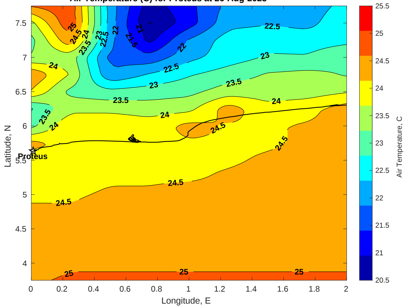
Air Temperature (C) for Proteus at 26-Aug-2025
