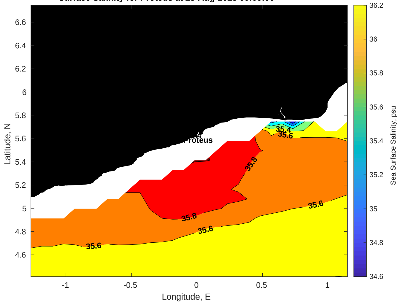
Surface Salinity for Proteus at 25-Aug-2025 00:00:00
