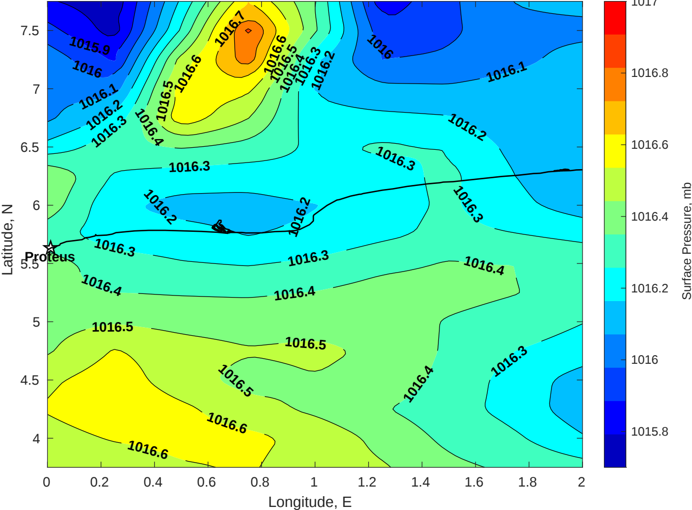
Surface Pressure (mb) for Proteus at 28-Aug-2025 00:00:00
