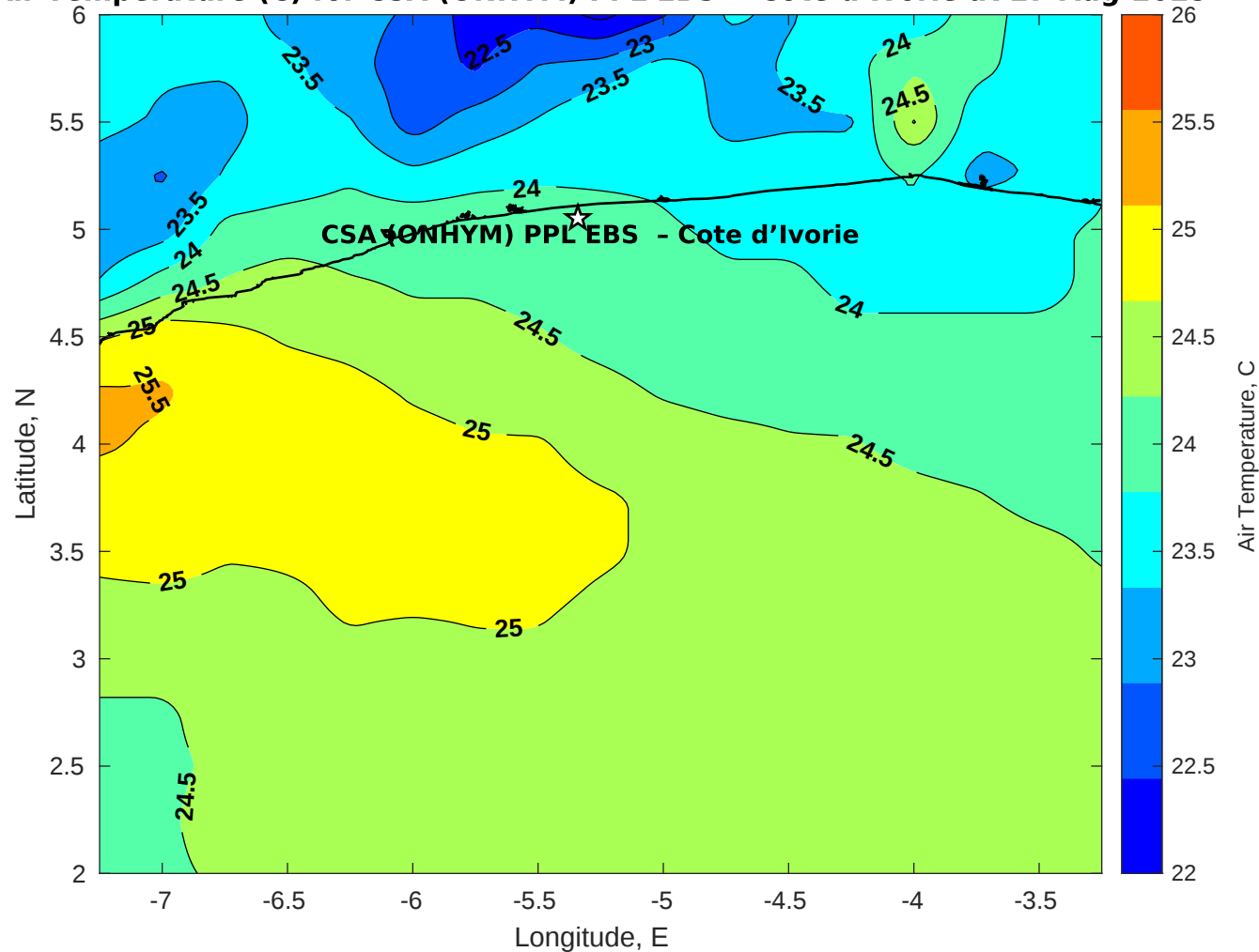
Air Temperature (C) for CSA (ONHYM) PPL EBS - Cote d'Ivoire at 27-Aug-2025
