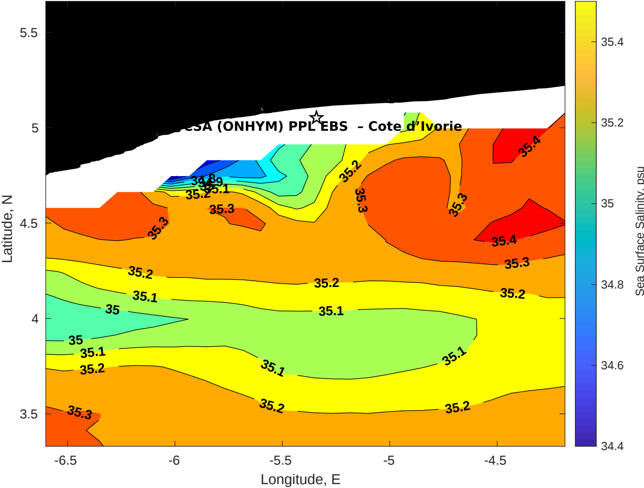
Surface Salinity for CSA (ONHYM) PPL EBS - Cote d'Ivoire at 26-Aug-2025 00:00:00
