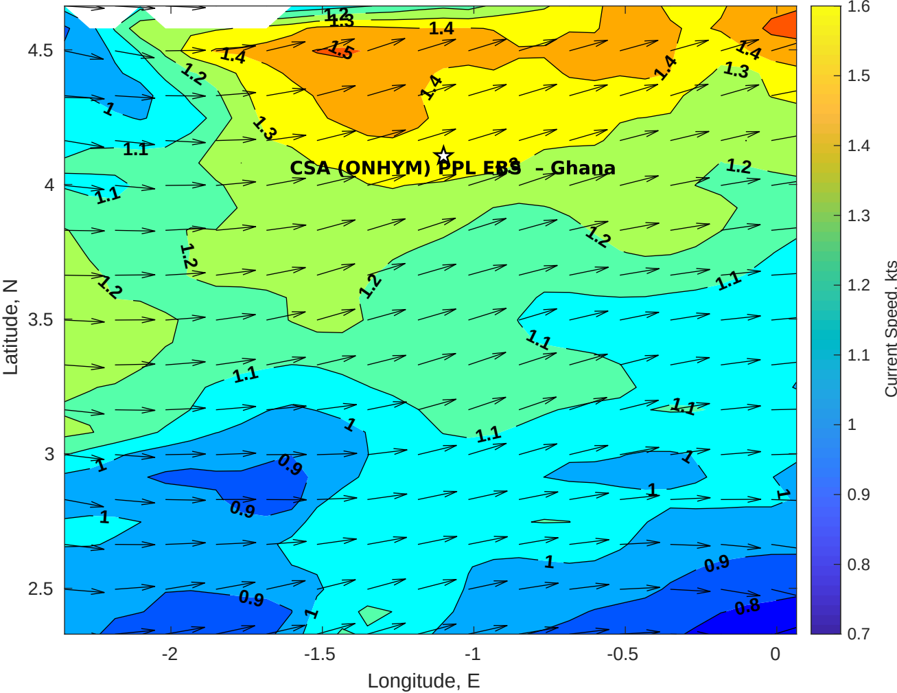
Surface Currents for CSA (ONHYM) PPL EBS - Ghana at 26-Aug-2025 00:00:00
