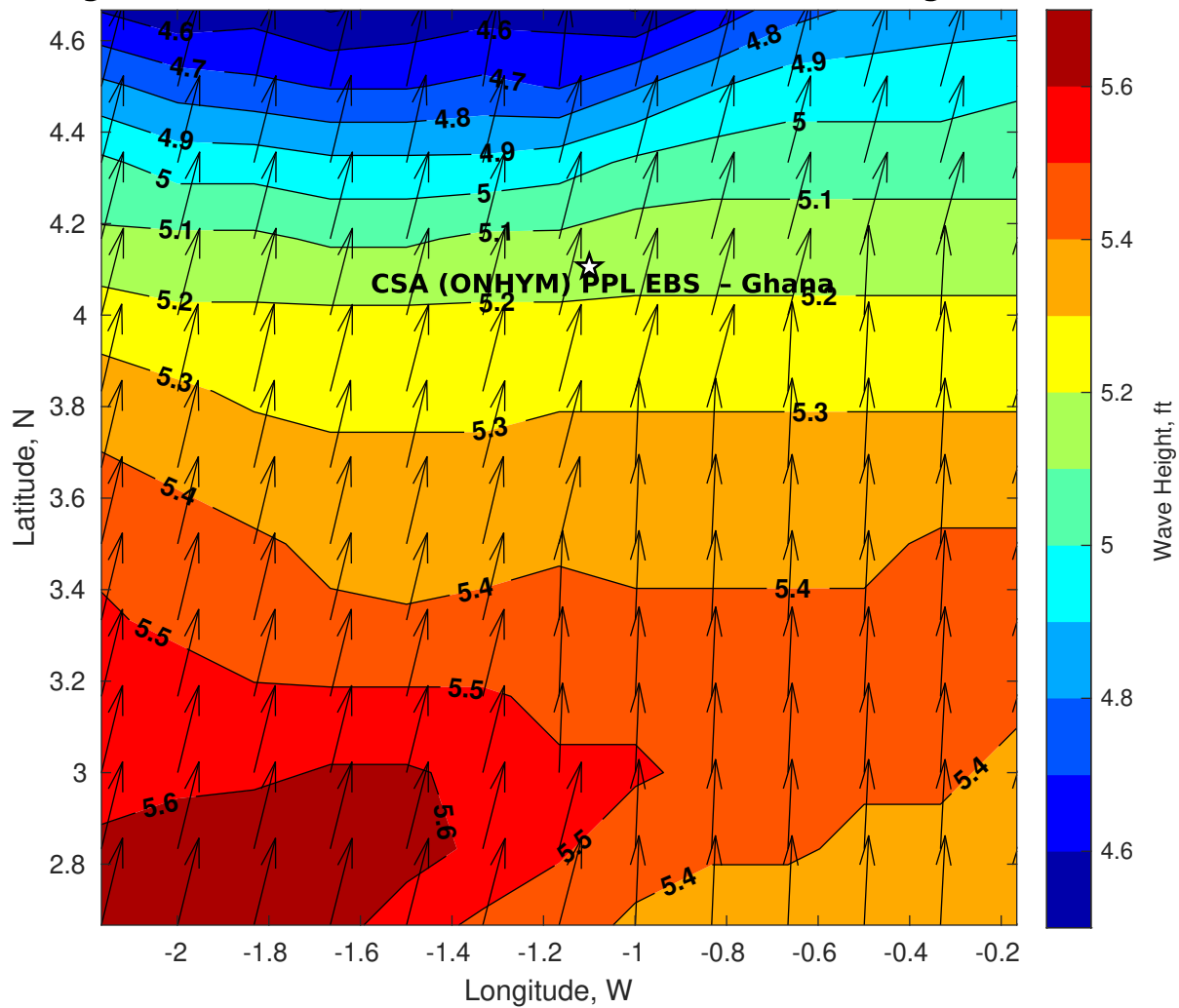
Wave Height (ft) for CSA (ONHYM) PPL EBS - Ghana at 27-Aug-2025 09:00:00
