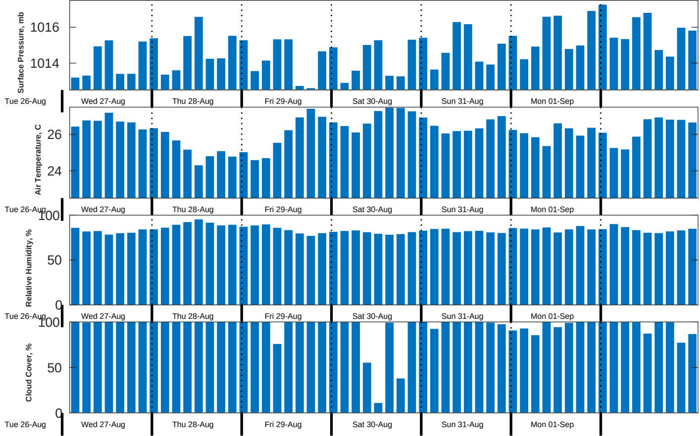
Met Forecast for CSA (ONHYM) PPL EBS - Guinea from 27-Aug-2025 00:00:00 to 03-Sep-2025 00:00:00
