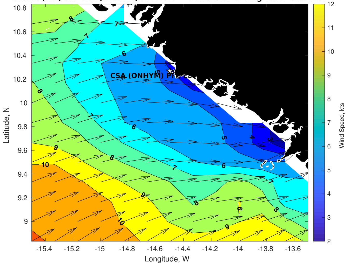
Winds (kts) for CSA (ONHYM) PPL EBS - Guinea at 27-Aug-2025 09:00:00
