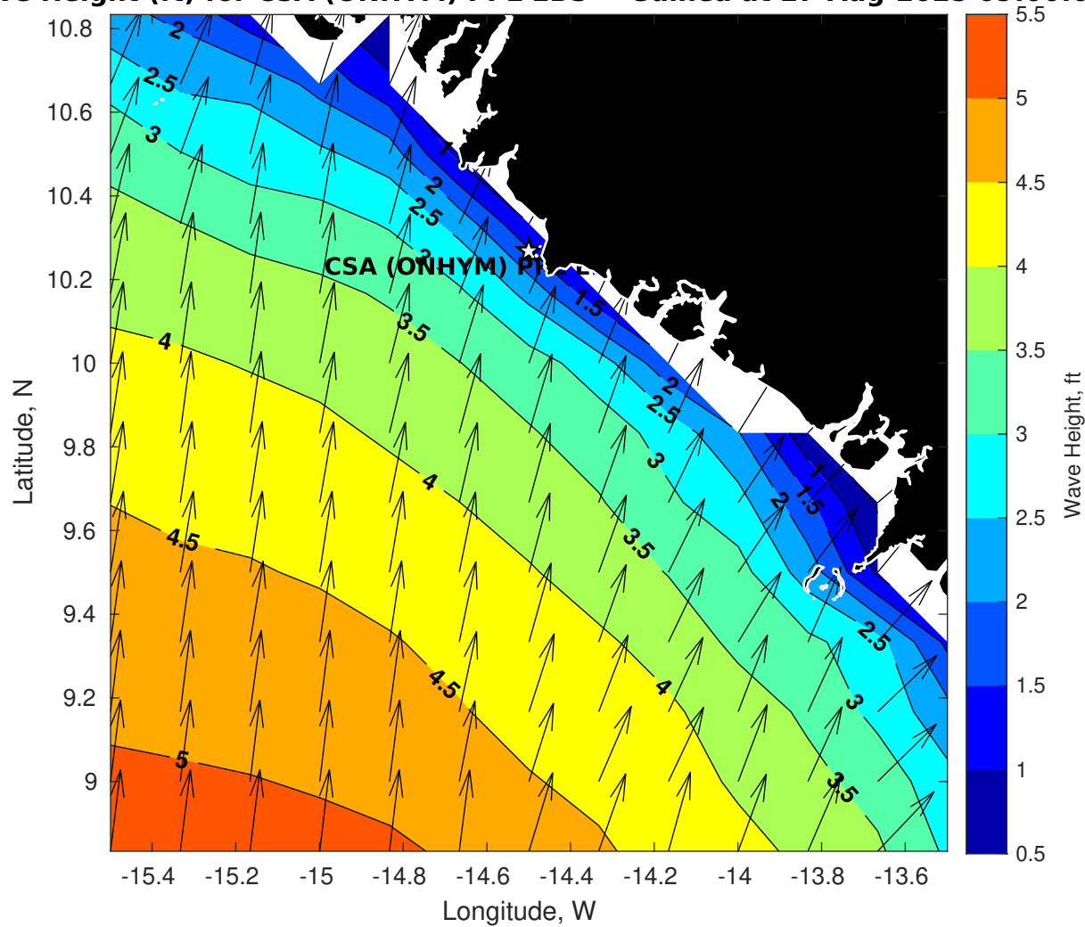
Wave Height (ft) for CSA (ONHYM) PPL EBS - Guinea at 27-Aug-2025 09:00:00
