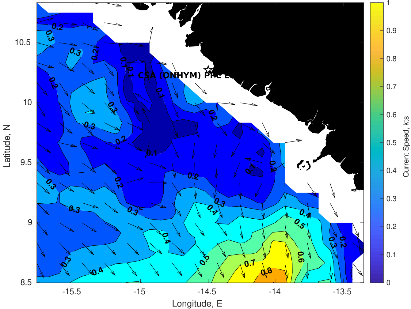
Surface Currents for CSA (ONHYM) PPL EBS - Guinea at 26-Aug-2025 00:00:00
