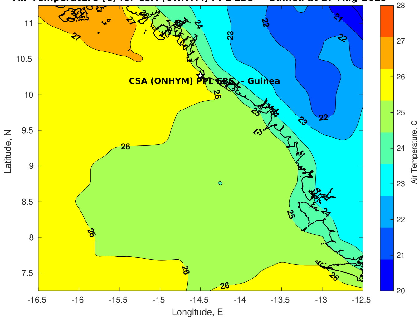
Air Temperature (C) for CSA (ONHYM) PPL EBS - Guinea at 27-Aug-2025
