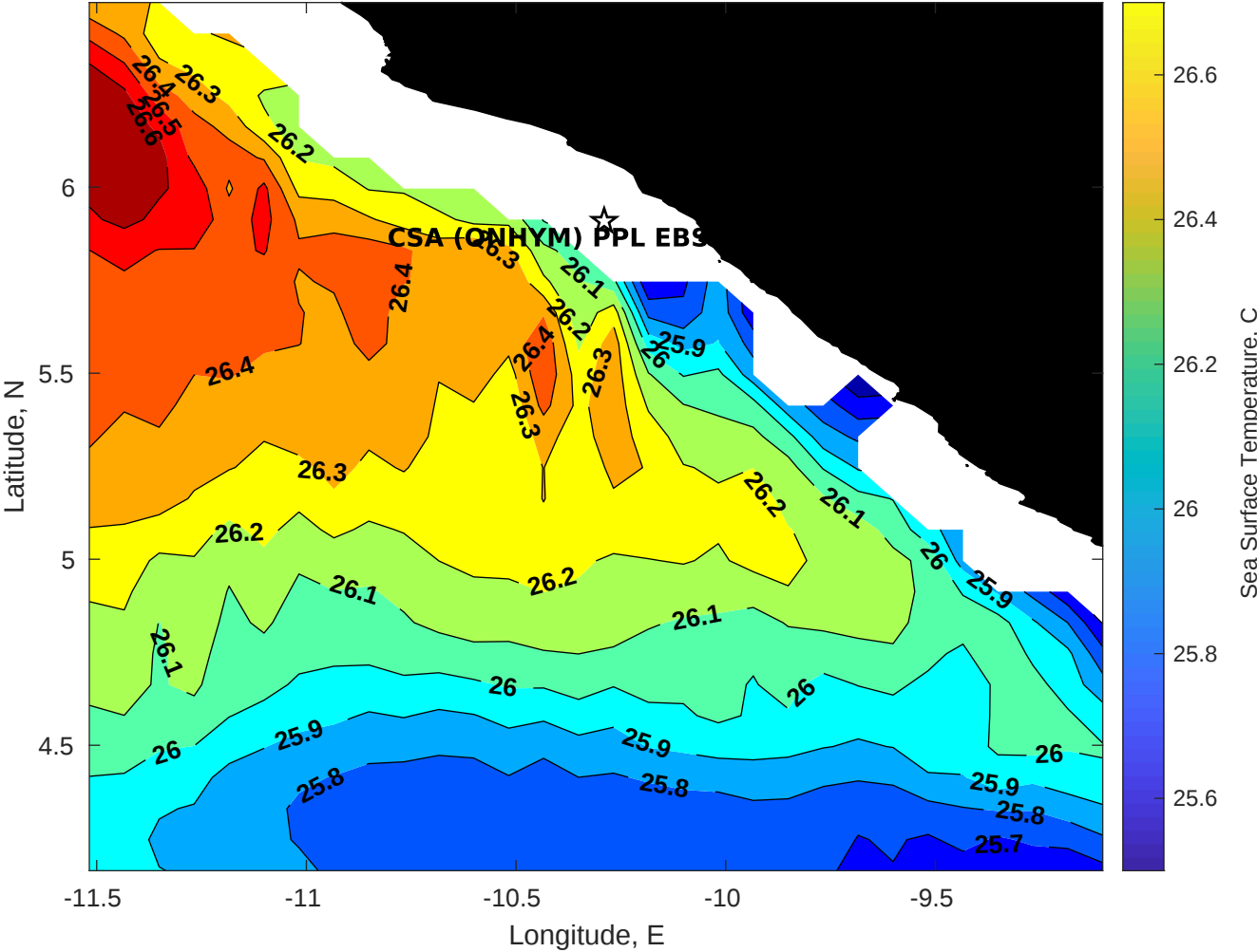
SST for CSA (ONHYM) PPL EBS - Liberia at 26-Aug-2025 00:00:00
