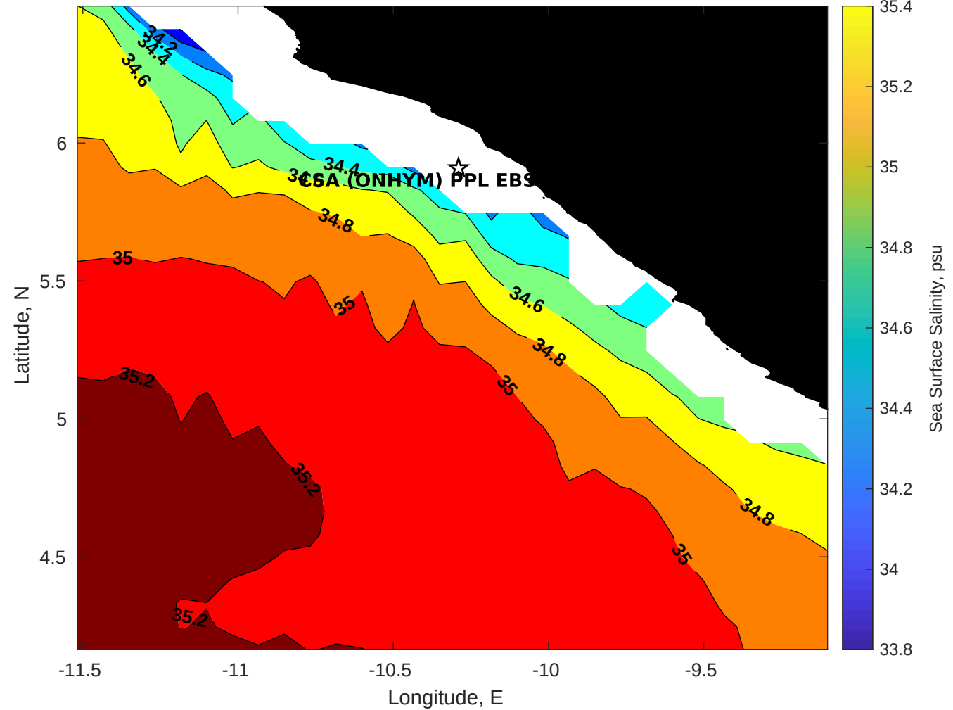
Surface Salinity for CSA (ONHYM) PPL EBS - Liberia at 26-Aug-2025 00:00:00
