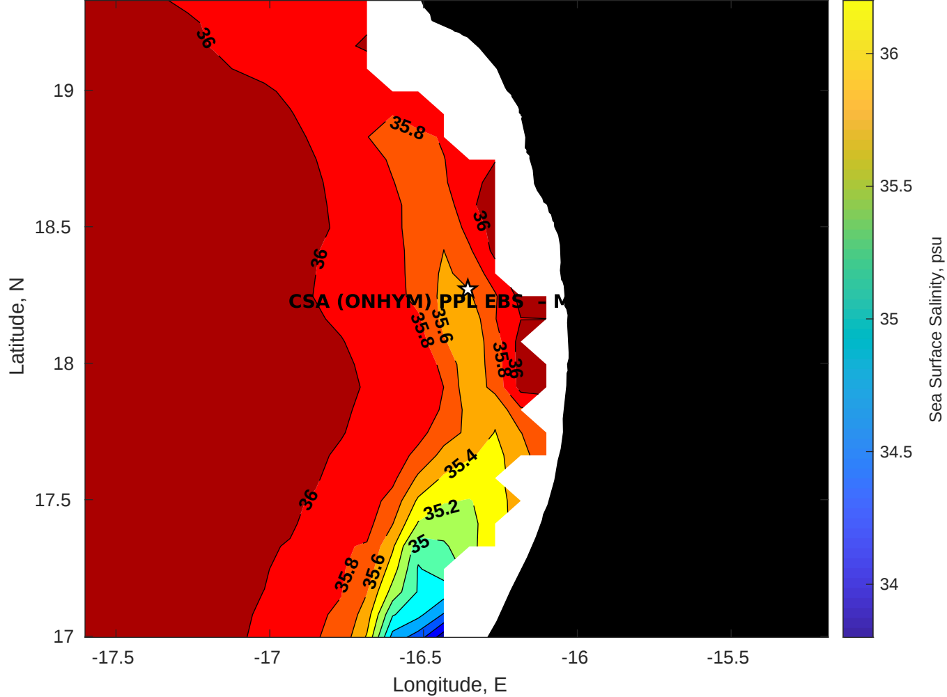
Surface Salinity for CSA (ONHYM) PPL EBS - Mauritania at 26-Aug-2025 00:00:00
