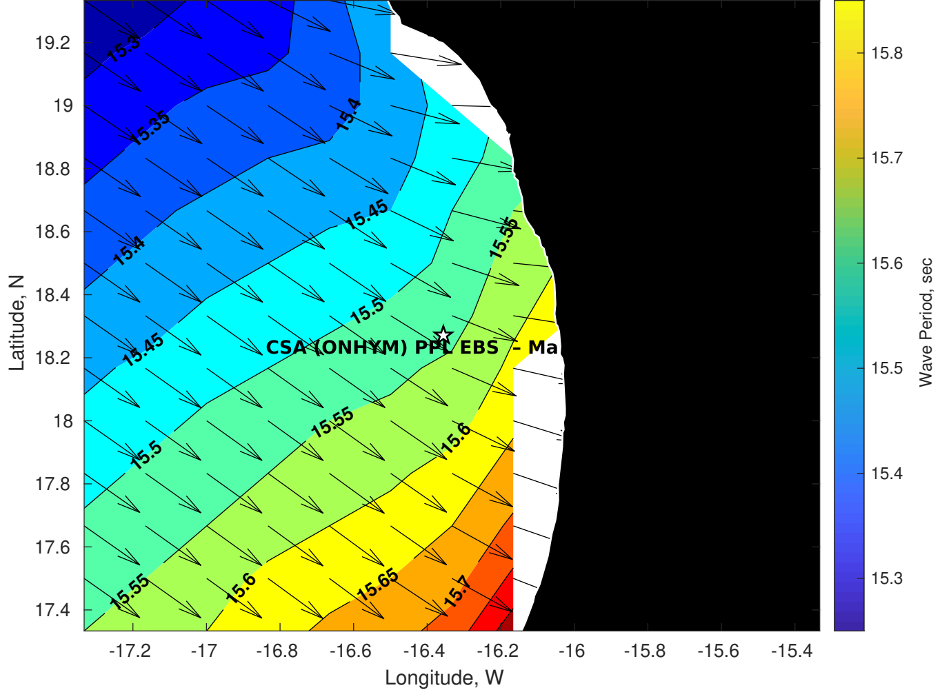
Wave Period (sec) for CSA (ONHYM) PPL EBS - Mauritania at 27-Aug-2025 09:00:00
