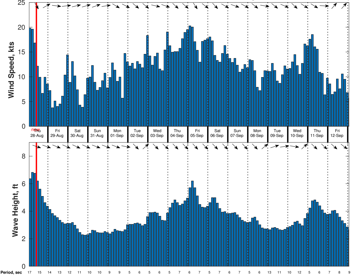
Wind & Wave Forecast for CSA (ONHYM) PPL EBS - Mauritania from 27-Aug-2025 01:00:00 to 12-Sep-2025 01:00:00
