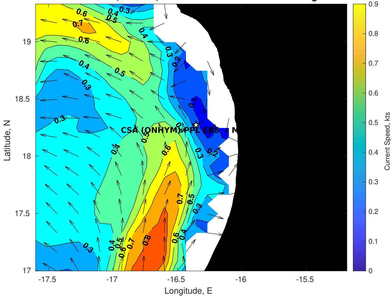
Surface Currents for CSA (ONHYM) PPL EBS - Mauritania at 26-Aug-2025 00:00:00
