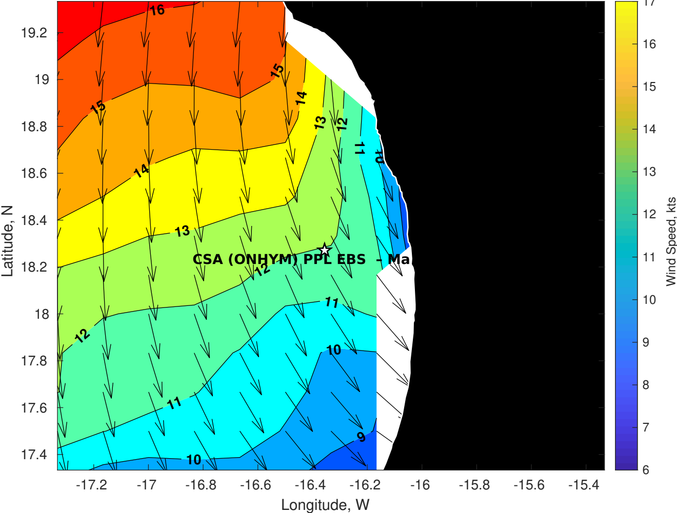
Winds (kts) for CSA (ONHYM) PPL EBS - Mauritania at 27-Aug-2025 09:00:00
